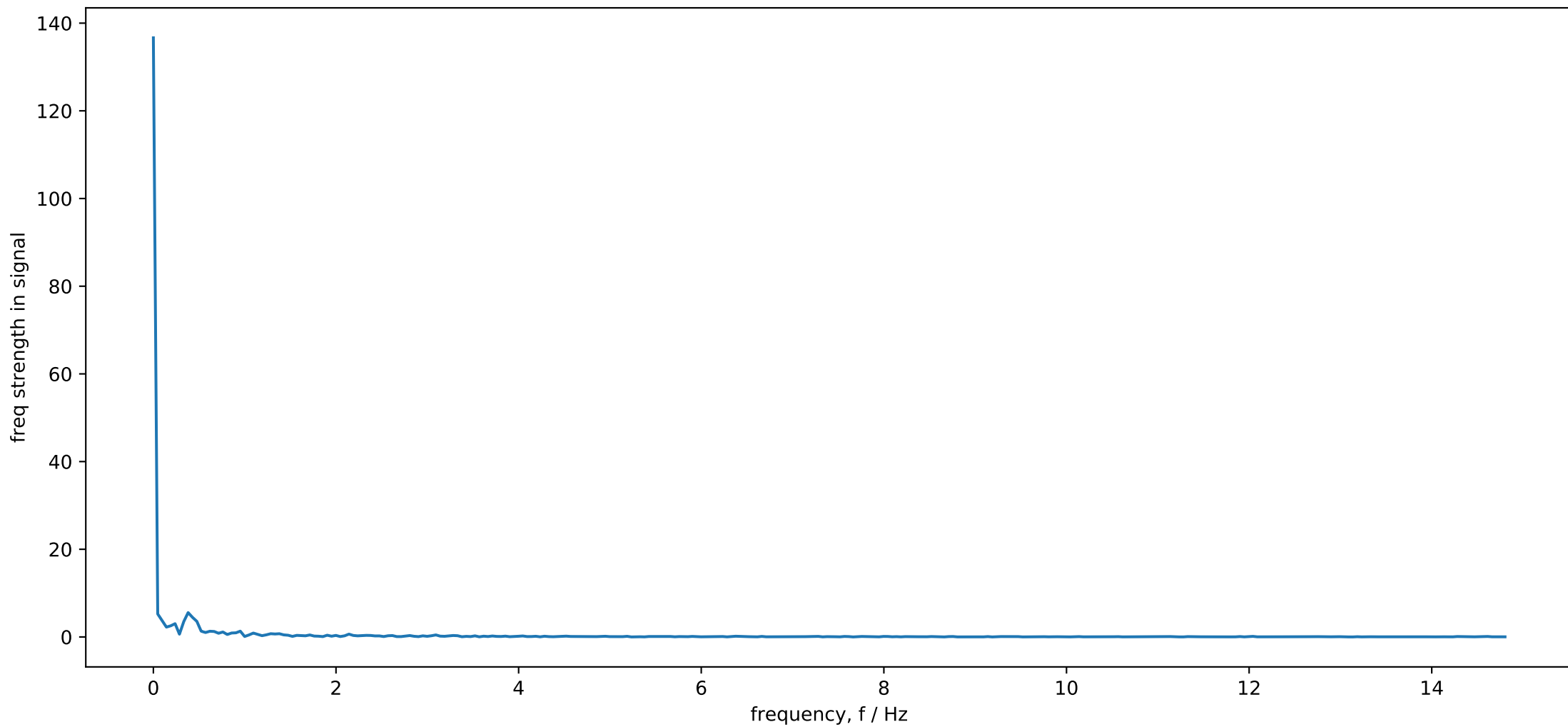
discrete FFT
