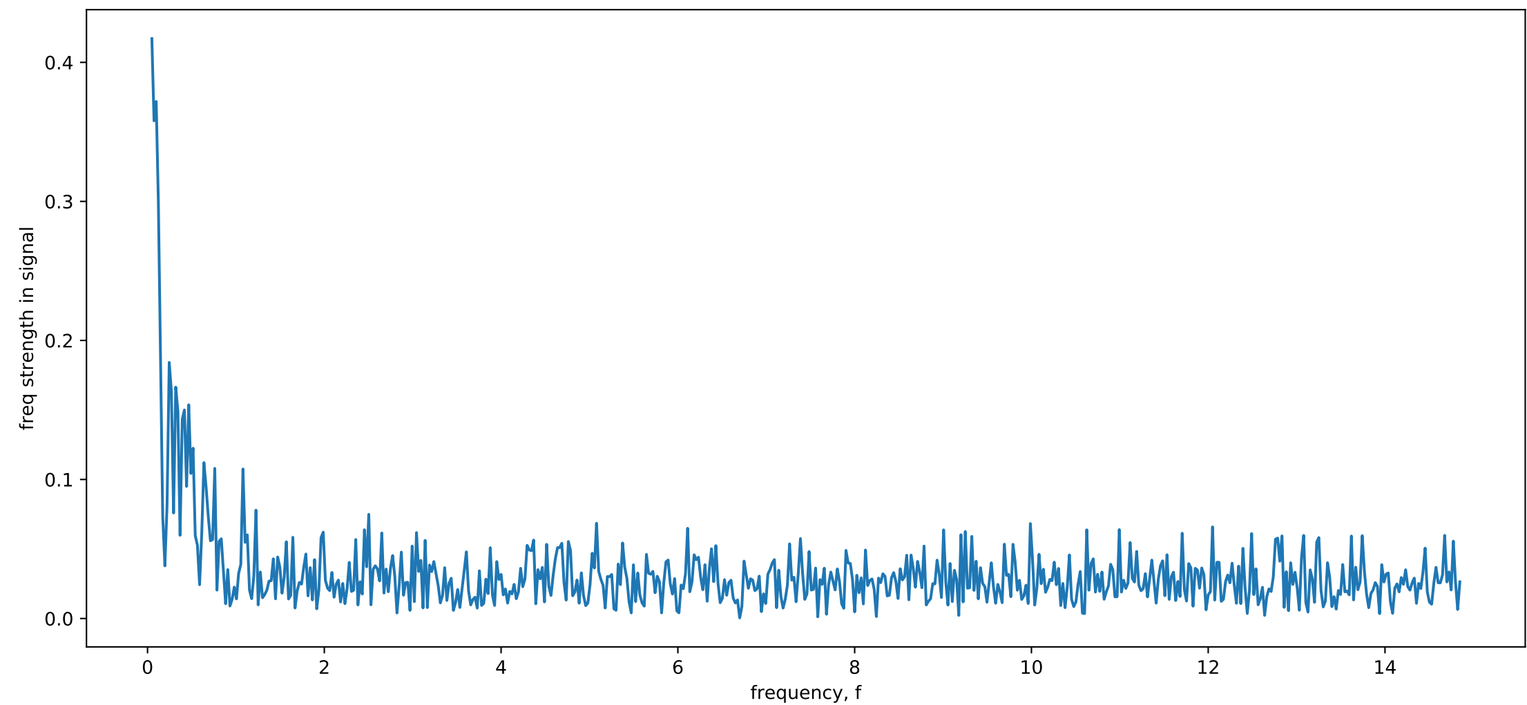
discrete FFT
