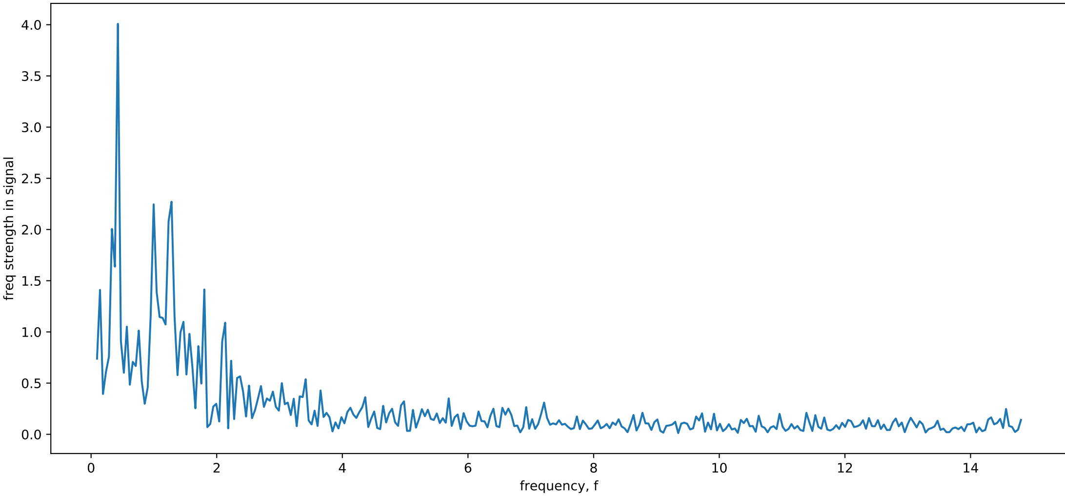
discrete FFT
