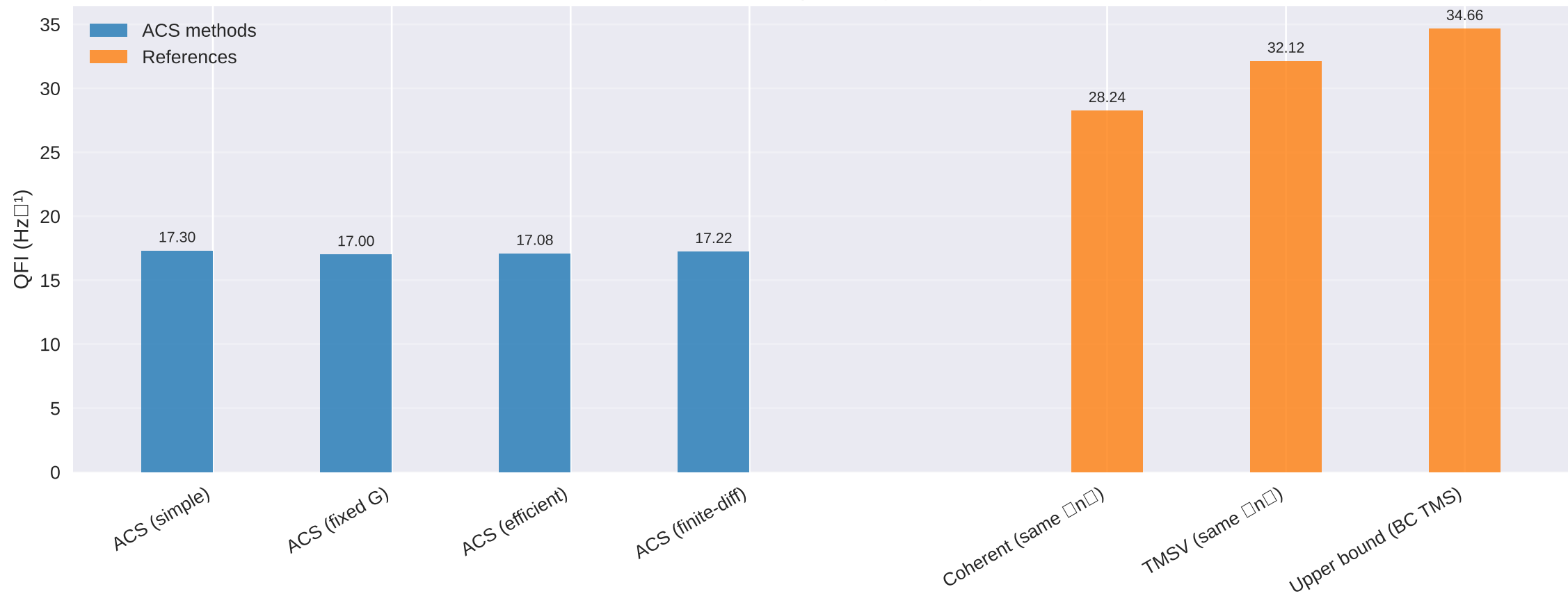
Final QFI Comparison (t = 10.0 s)
