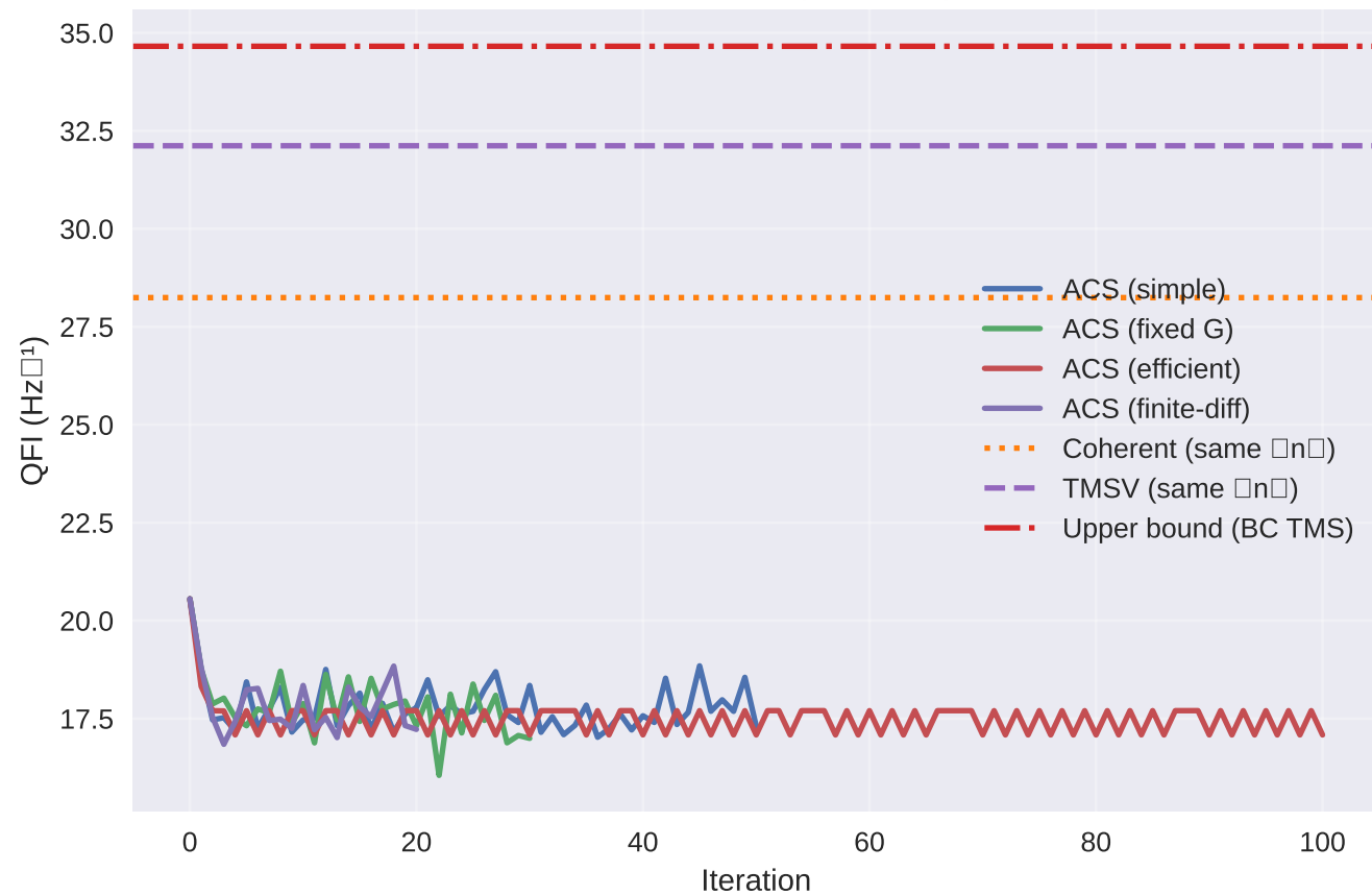
QFI vs Iteration (t = 10.0 s)
