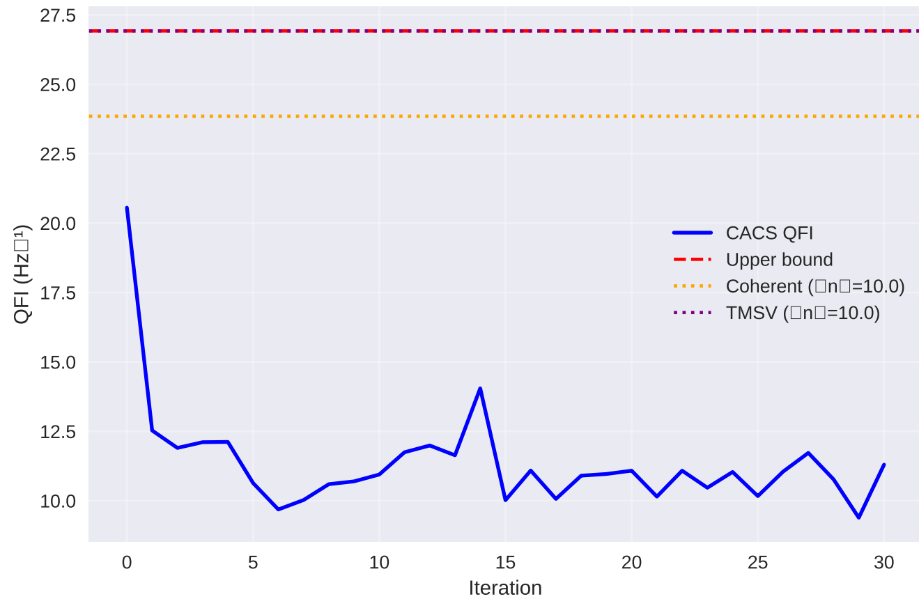
CACS Convergence ( \langle n \rangle \leq 10.0 )
