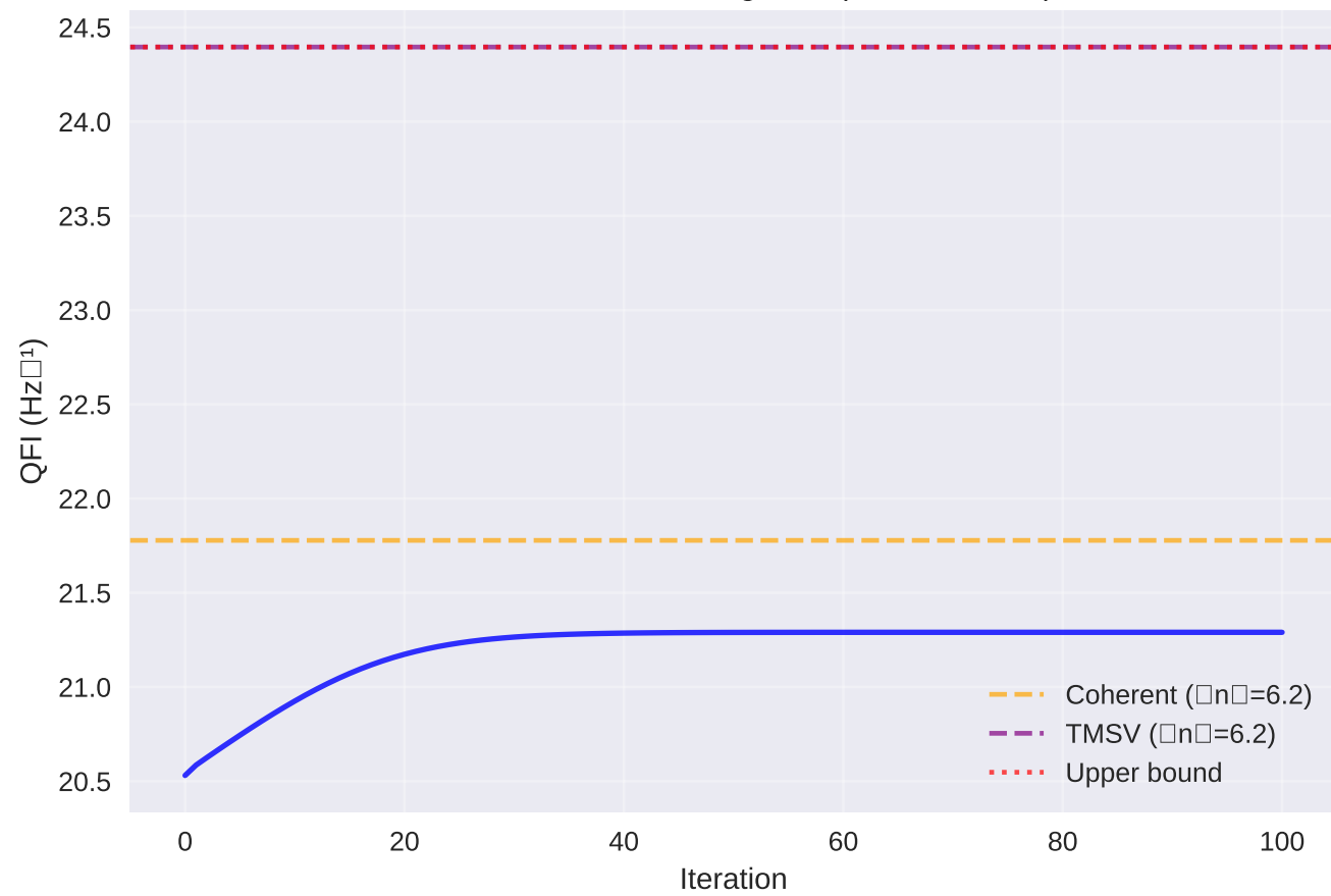
Convergence Rate
