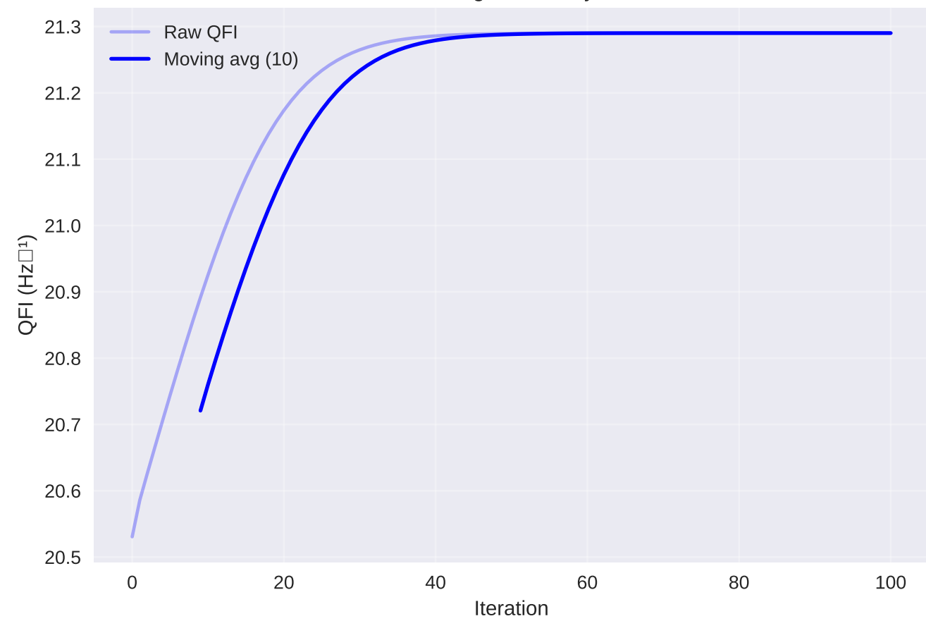
Convergence Analysis
