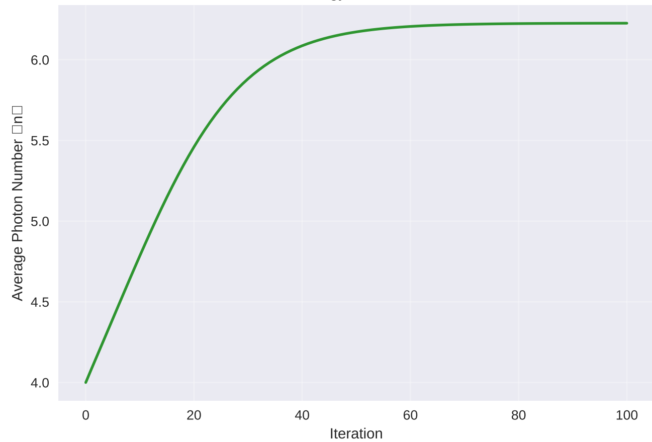
Convergence Analysis
