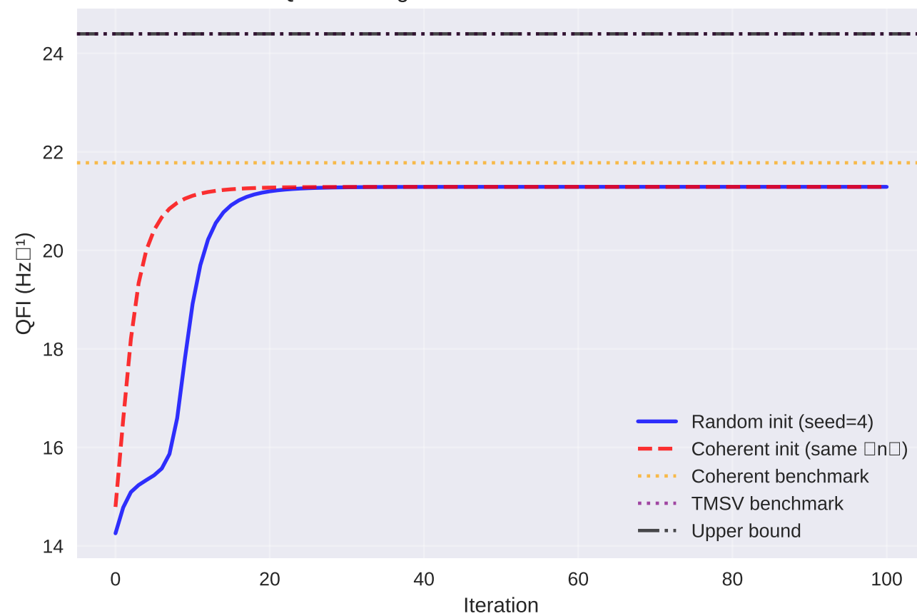
QFI Convergence: Random vs Coherent Init
