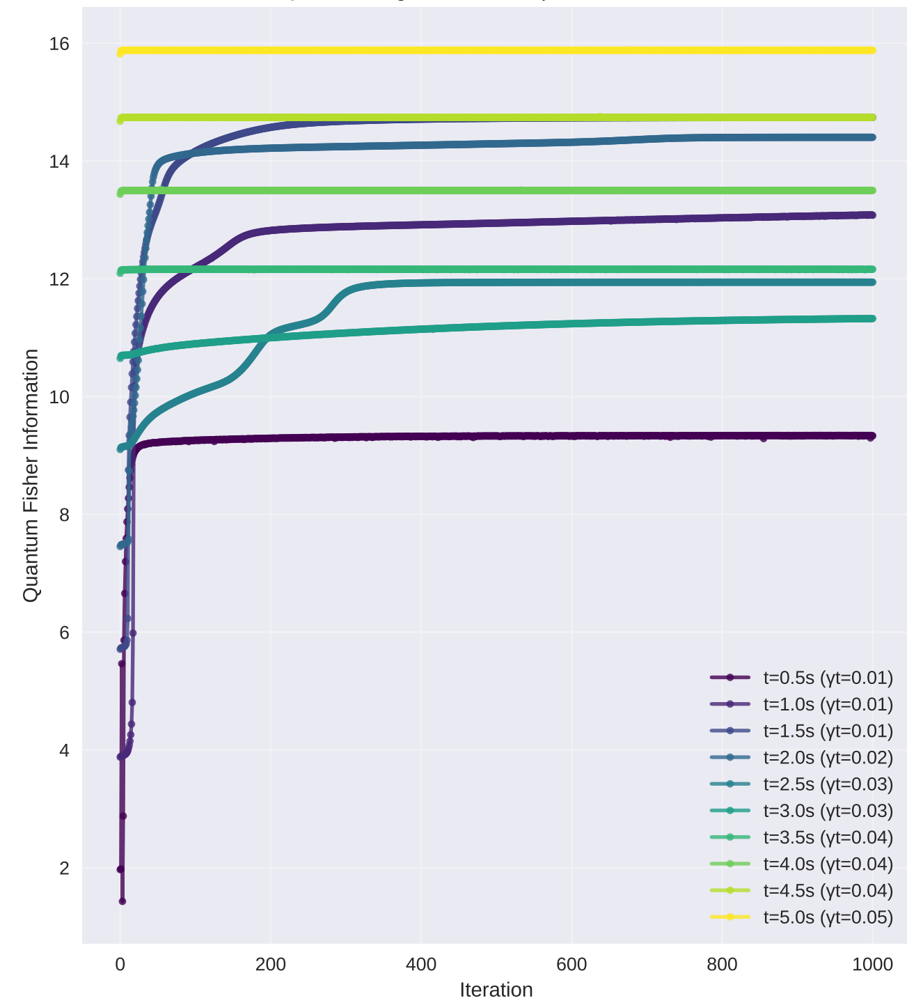
QFI Convergence for All Optimization Times
