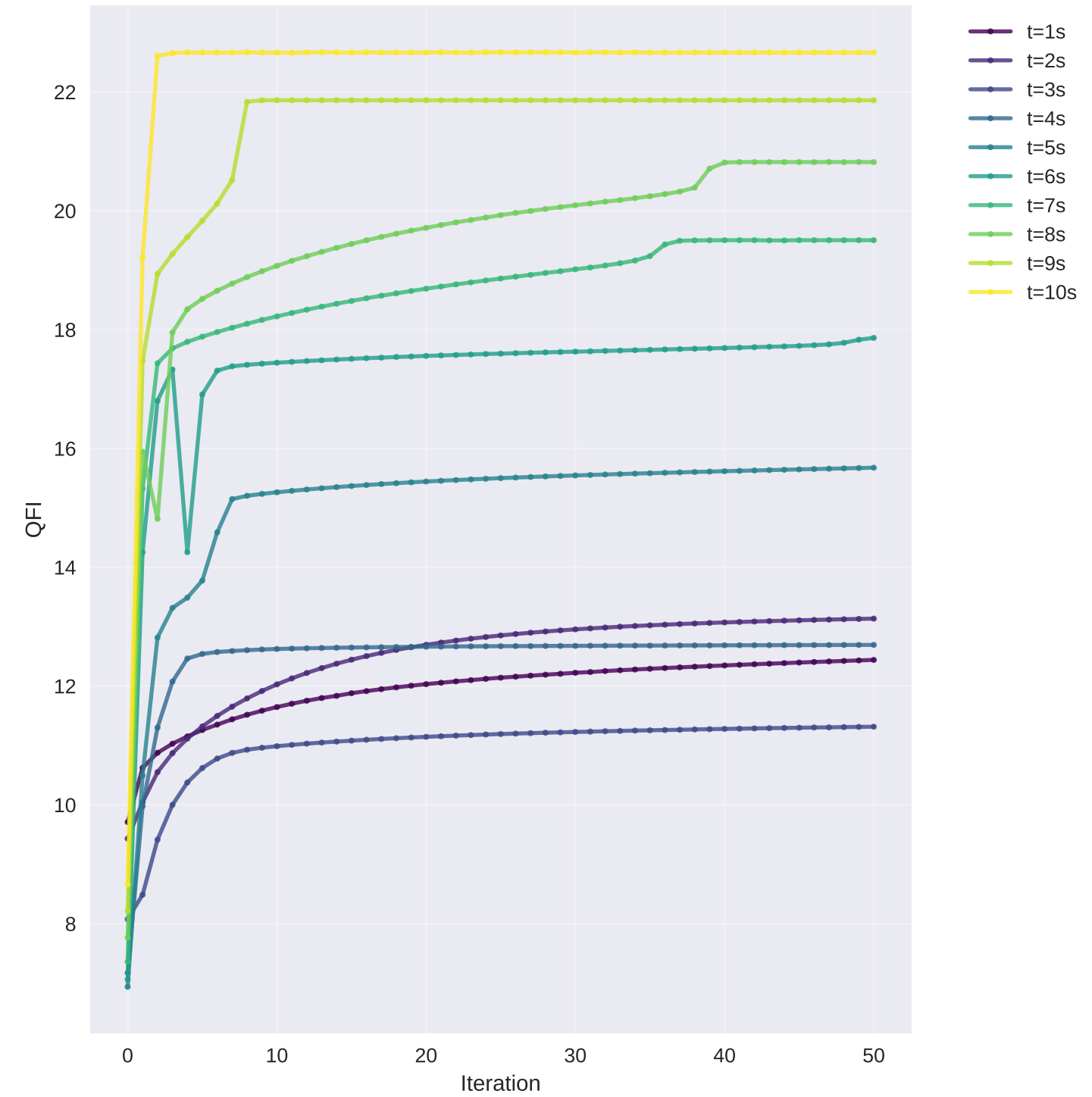
QFI Convergence for All Times
