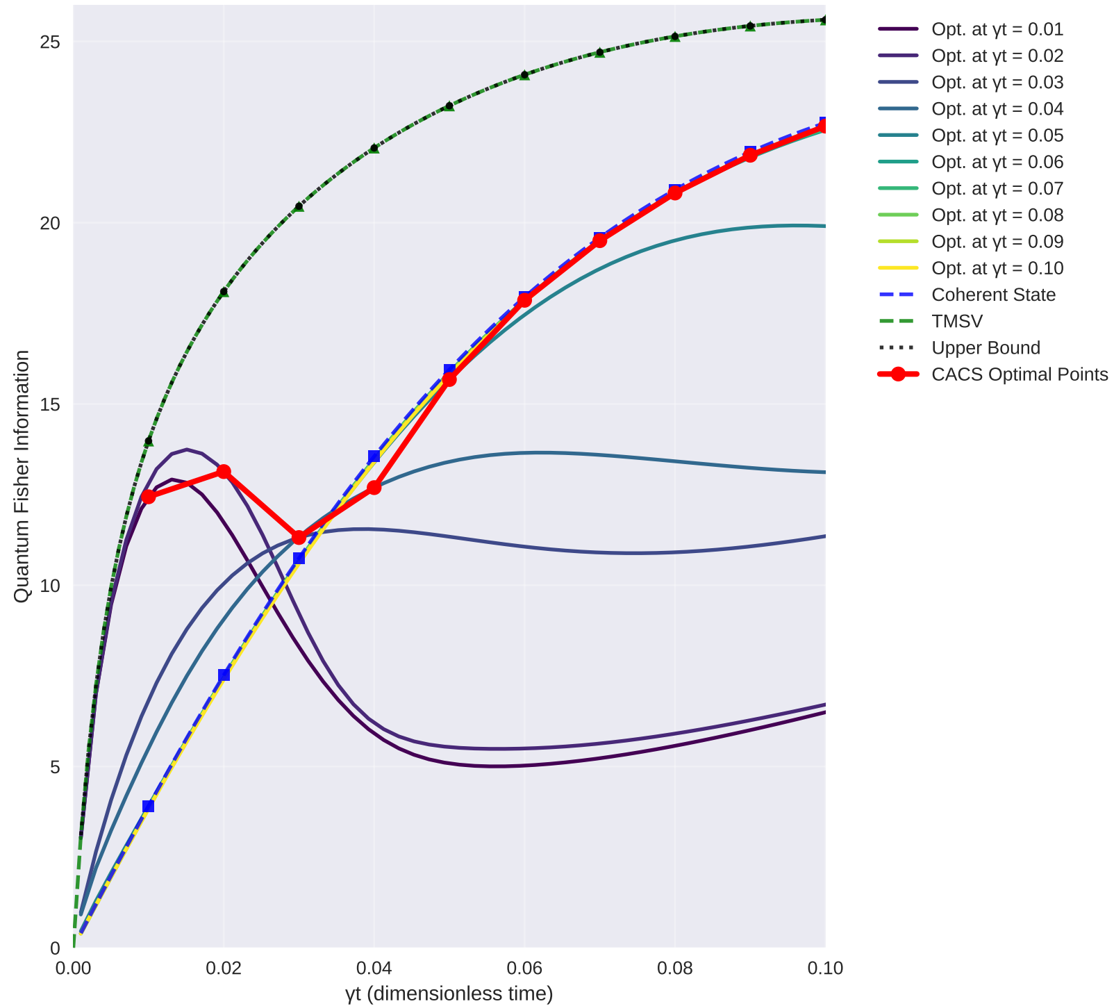
QFI Evolution and Benchmark Comparison
