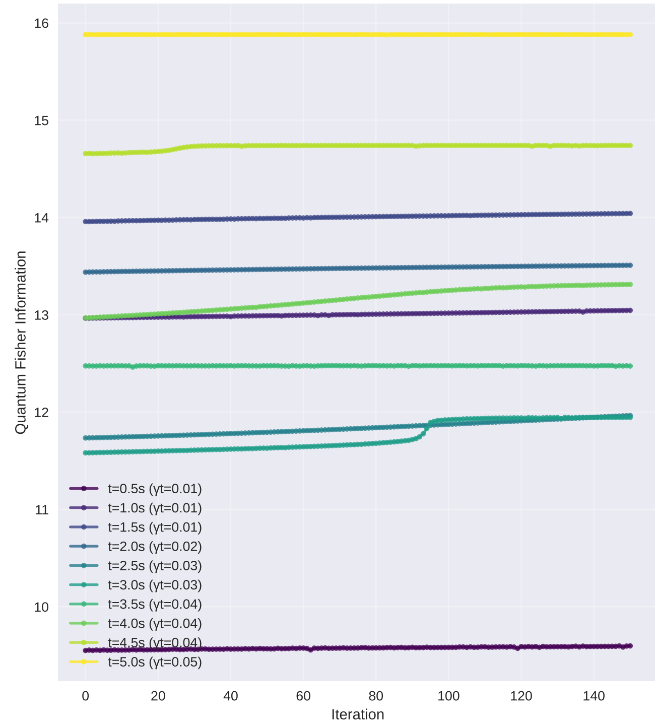
QFI Convergence for All Optimization Times
