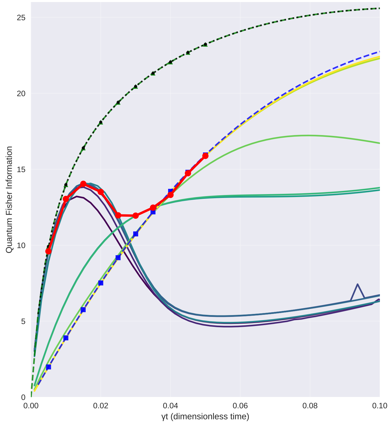
QFI Evolution and Benchmark Comparison
