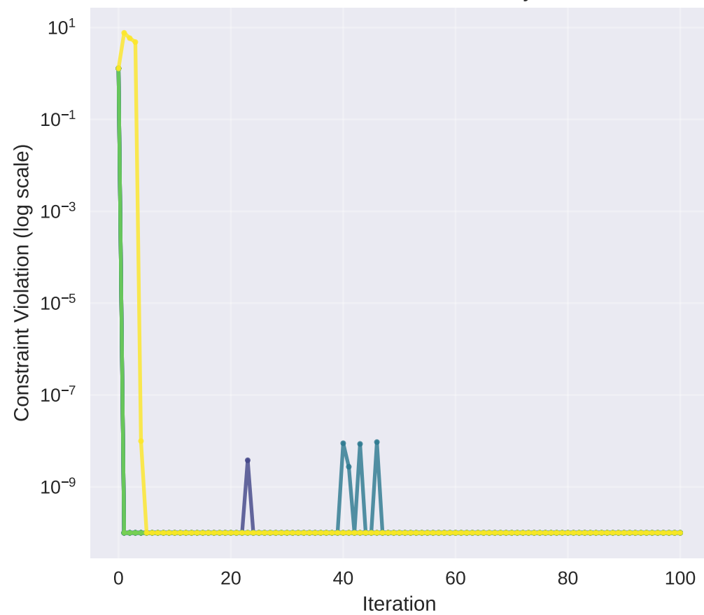
Constraint Violation History
