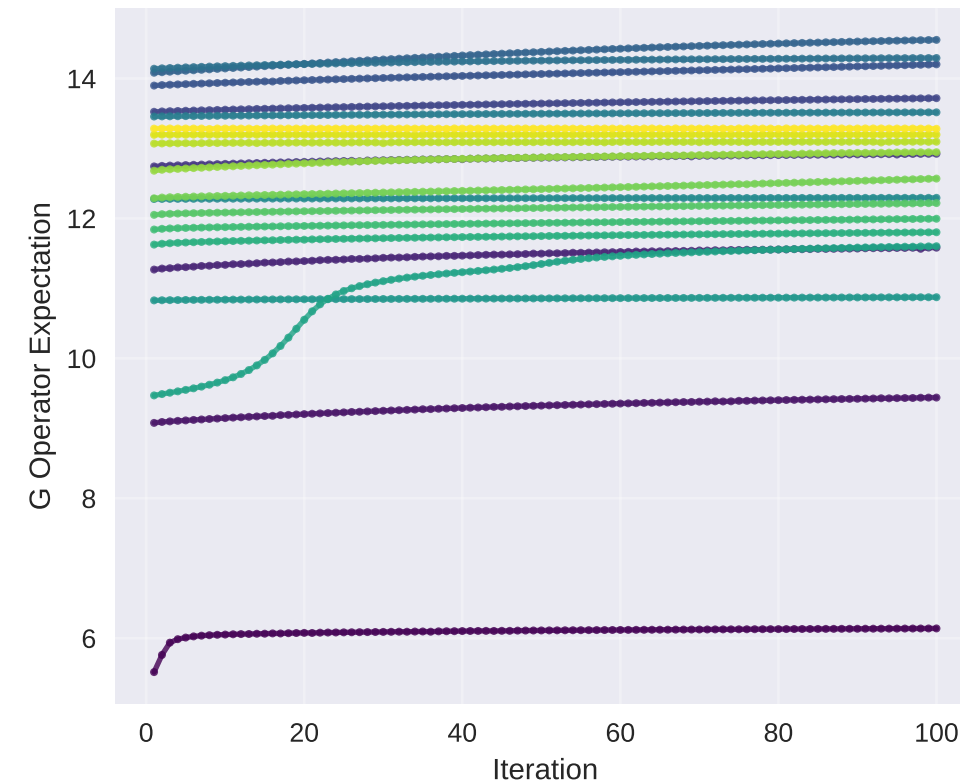
G Operator Evolution
