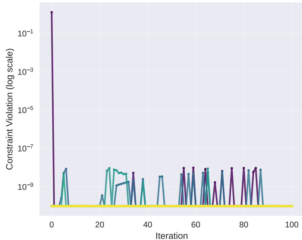
Constraint Violation History
