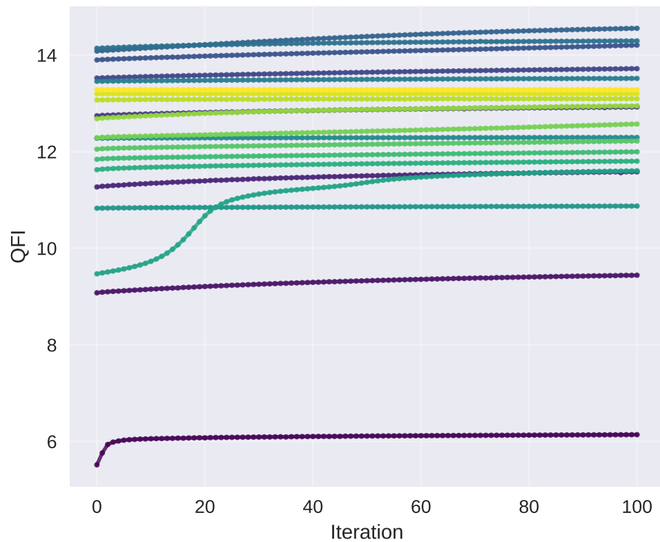
QFI Convergence for All Times
