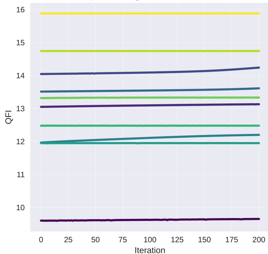
QFI Convergence for All Times
