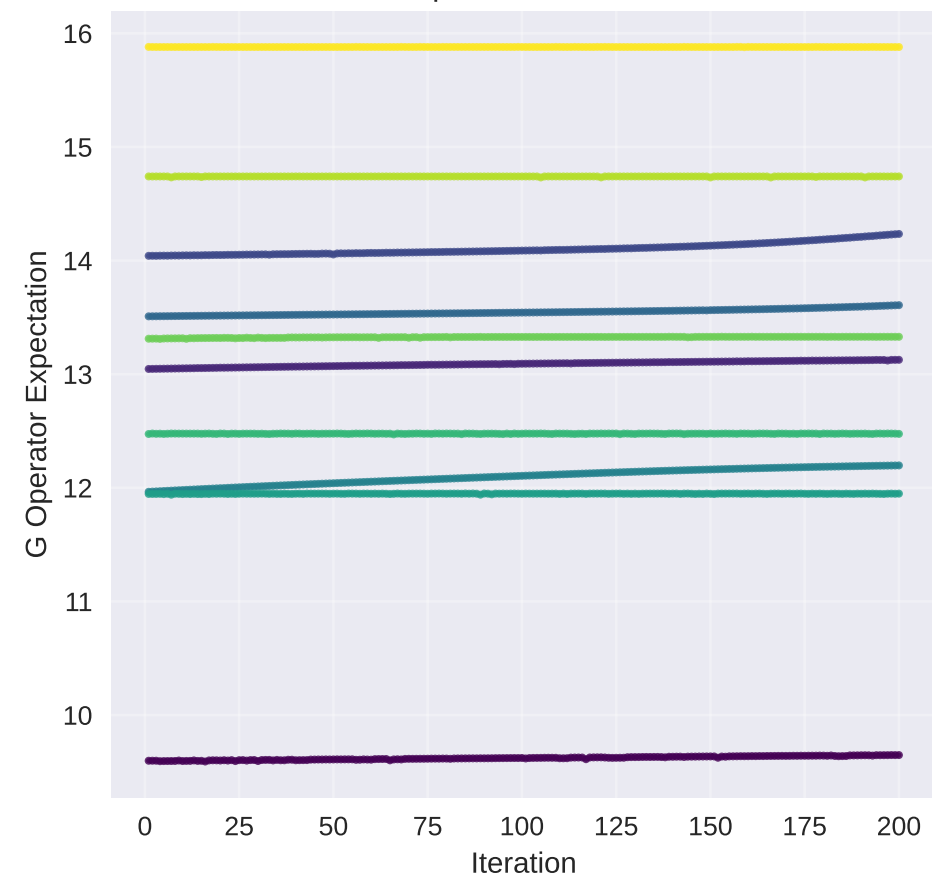
G Operator Evolution
