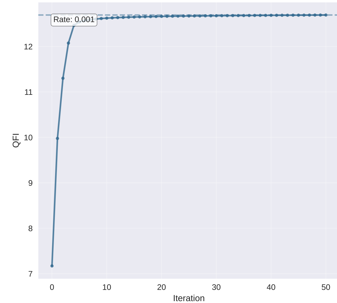
t = 4s (yt = 0.04) □ Not Converged Final QFI: 12.6924
