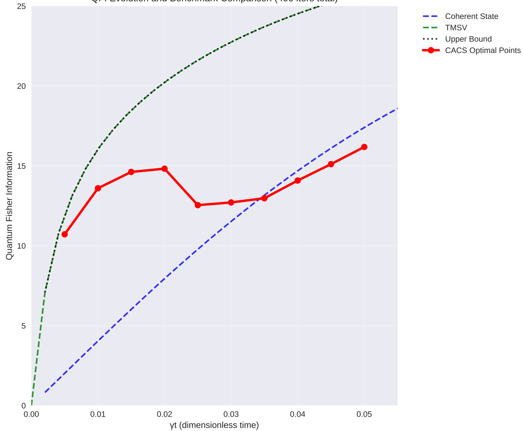
QFI Evolution and Benchmark Comparison (400 iters total)
