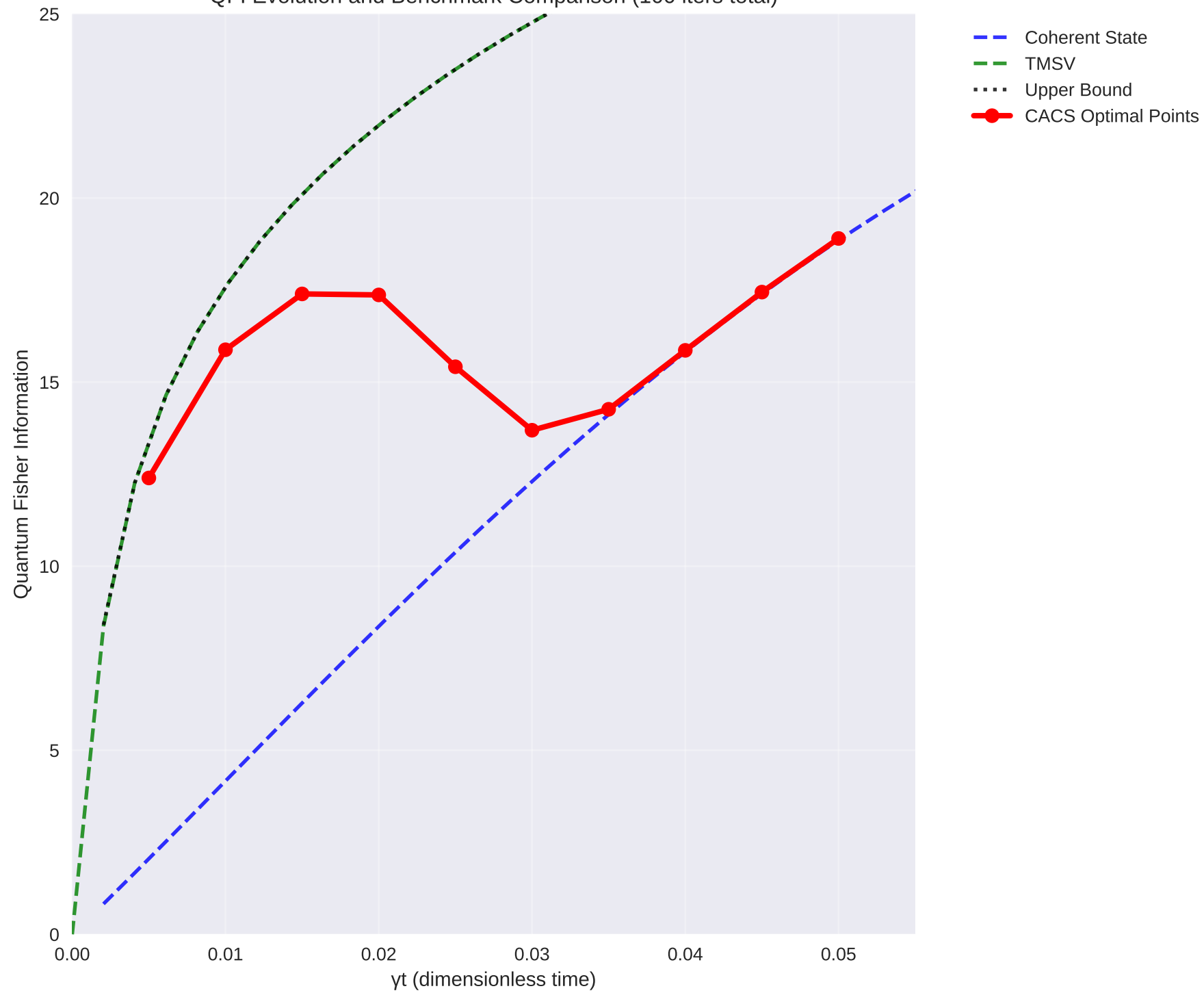
QFI Evolution and Benchmark Comparison (100 iters total)
