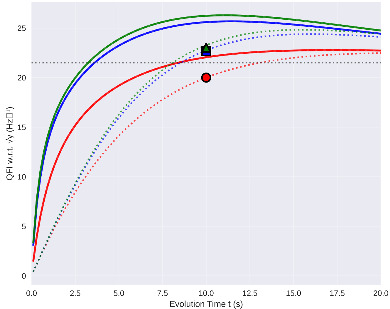
QFI vs Time: CACS Results vs Gaussian References
