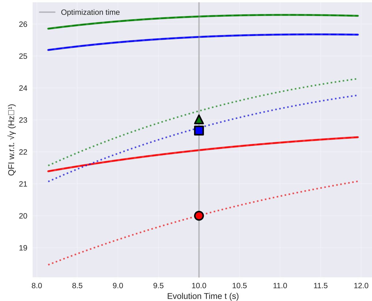
QFI vs Time: Zoomed View ( t = 8-12\text{s} )
