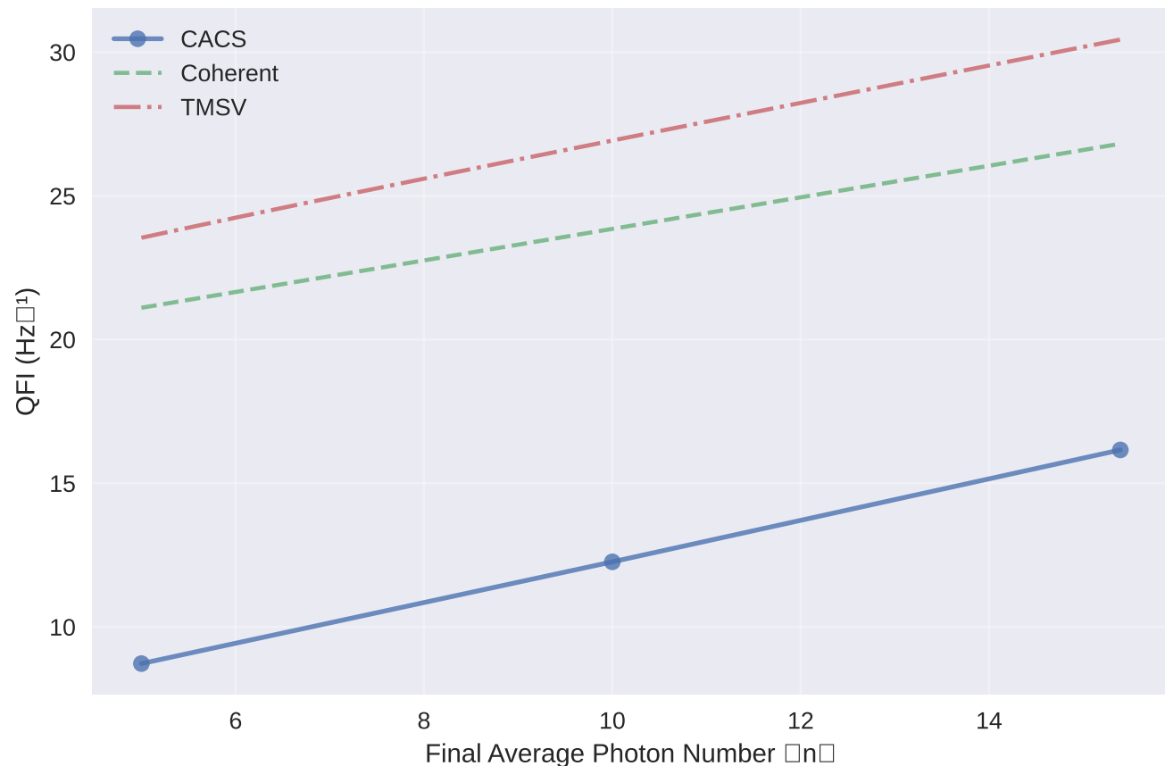
QFI vs Energy: CACS vs Gaussian States
