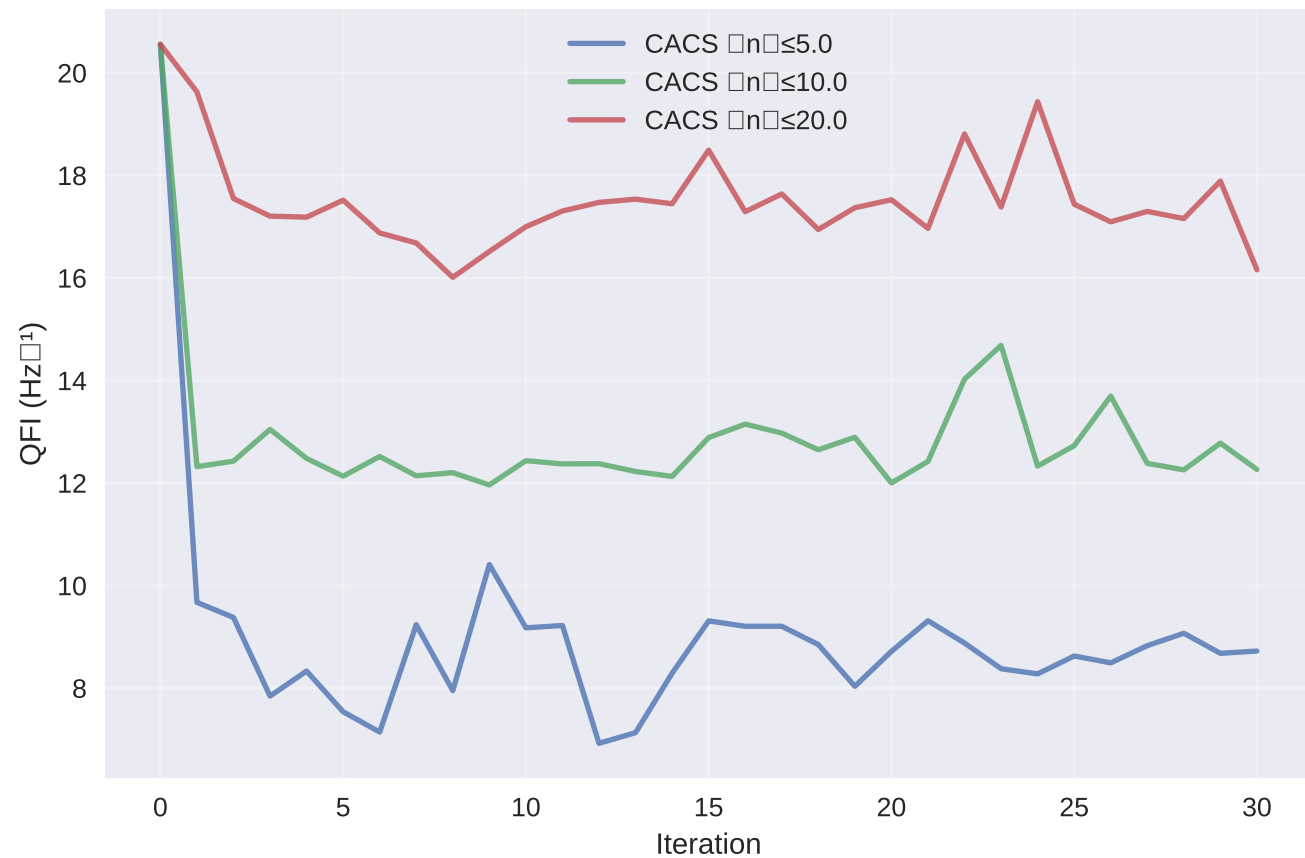
CACS Convergence (t = 10.0 s)
