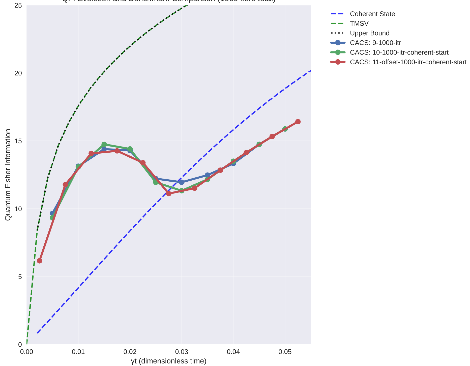
QFI Evolution and Benchmark Comparison (1000 iters total)
