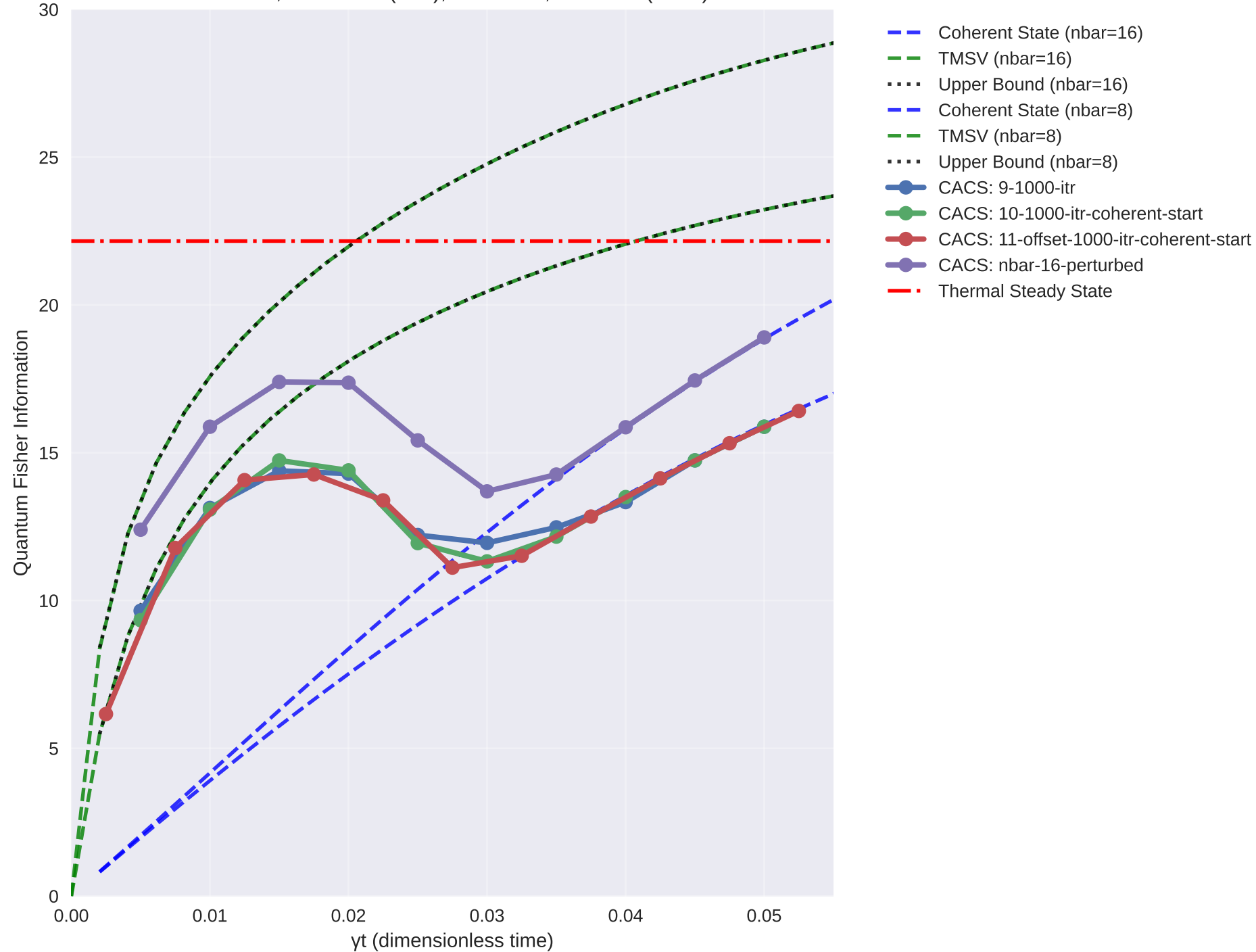
QFI Evolution and Benchmark Comparison nbar = 8, 1000 iters (3 hr); nbar = 16, 100 iters (13 hr)
