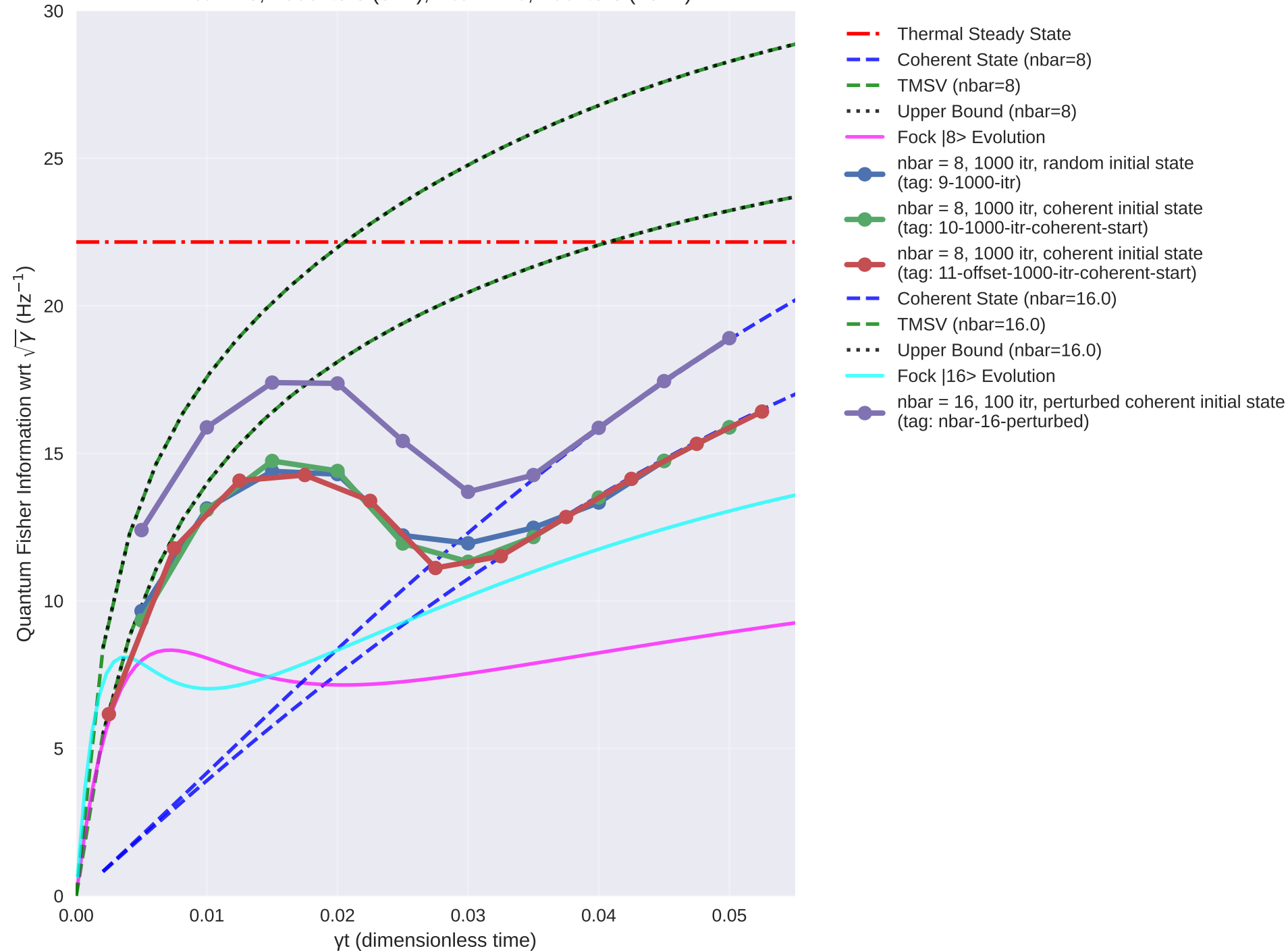
QFI Evolution and Benchmark Comparison n_{\text{bar}} = 8 , 1000 iters (3 hr); n_{\text{bar}} = 16 , 100 iters (13 hr)
