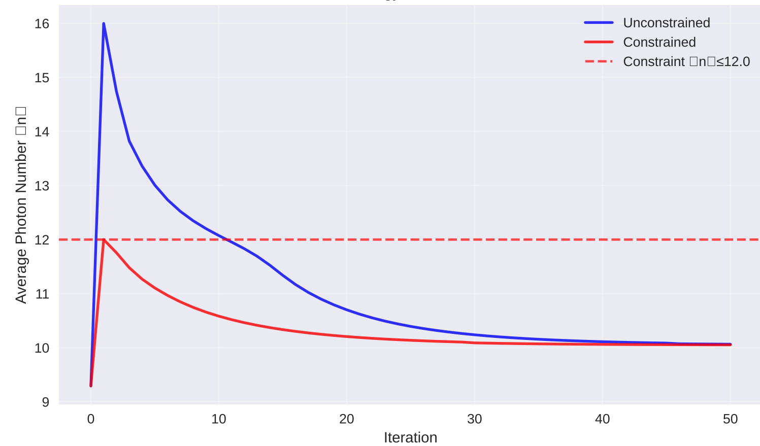
G Operator Expectation Evolution
