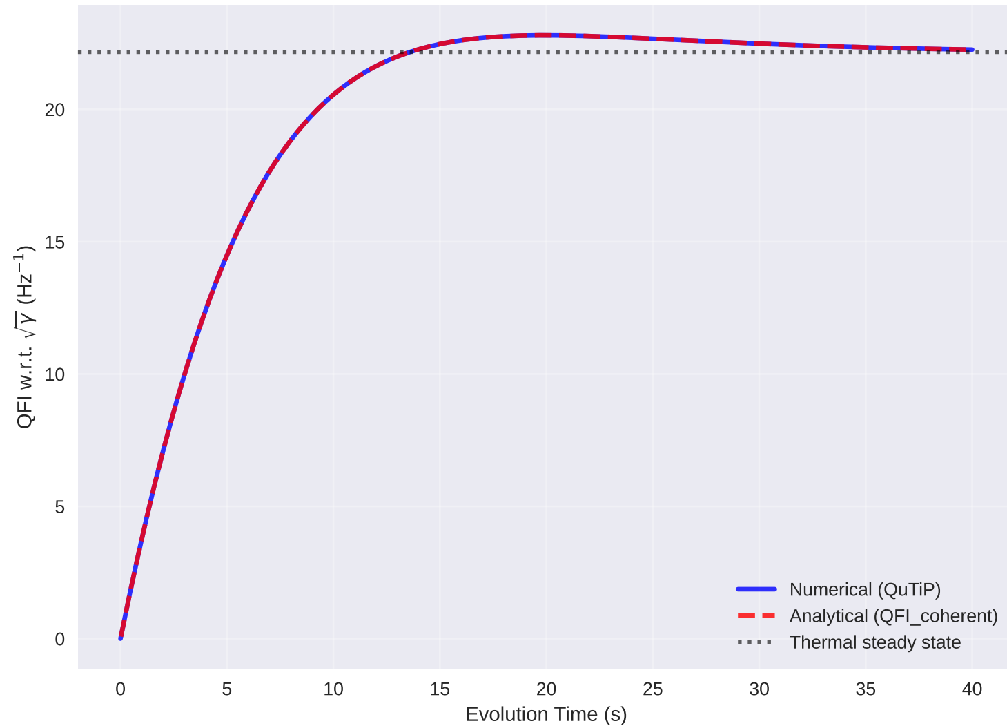
Coherent State QFI: Numerical vs Analytical ( \alpha=2.0 )
