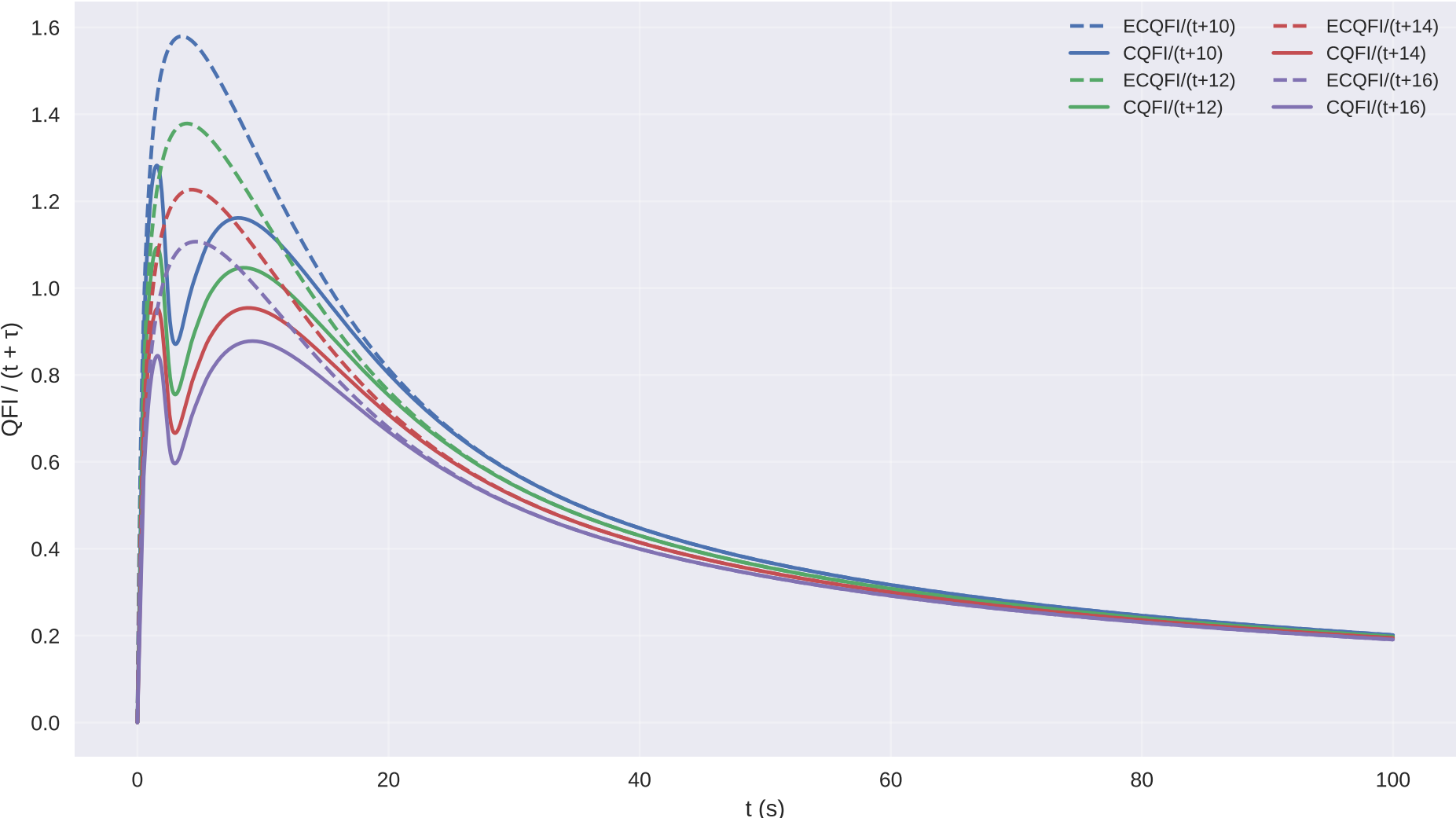
Scaled QFI for \tau = 10, 12, 14
