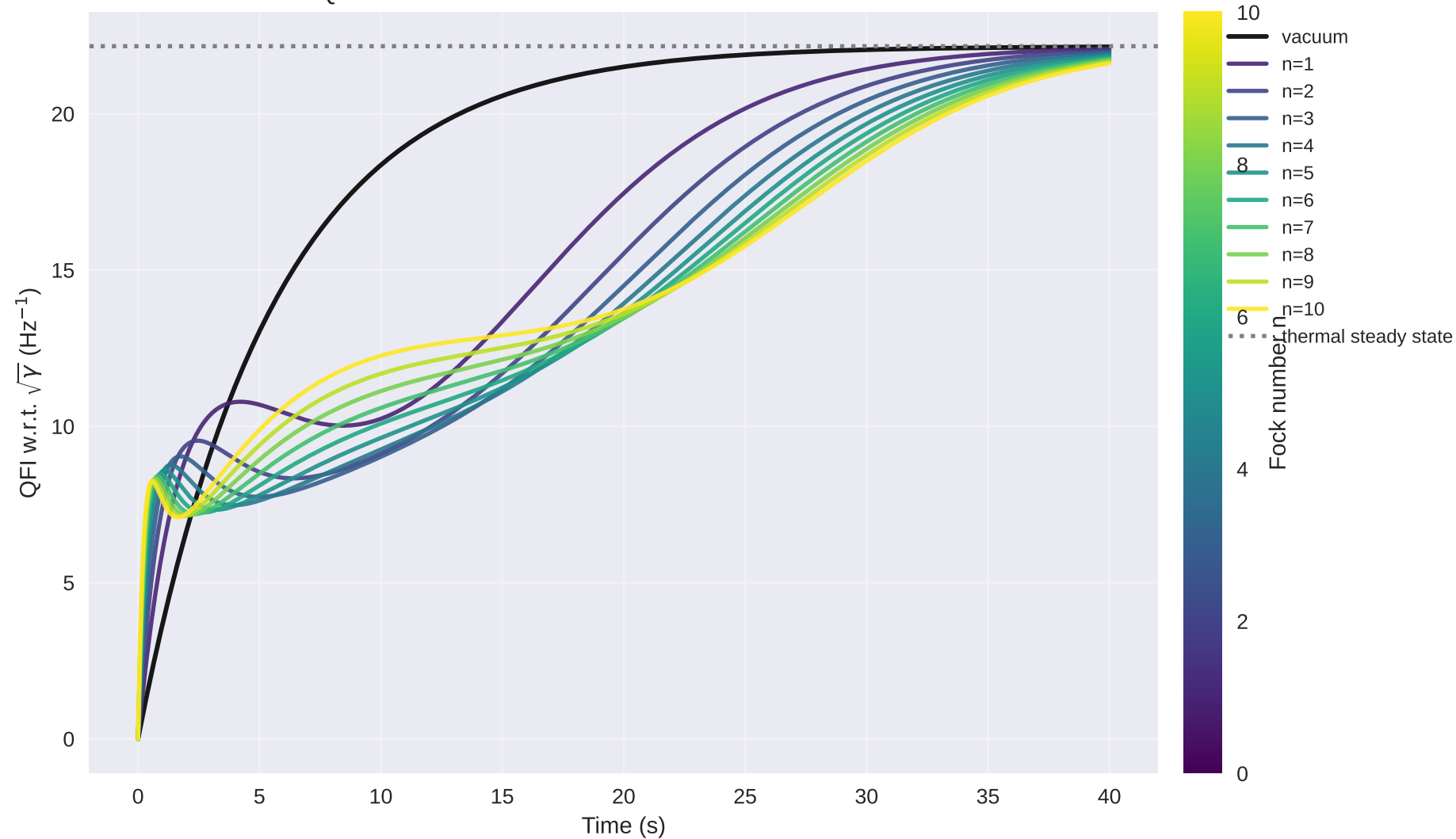
Quantum Fisher Information: Vacuum and Fock States
