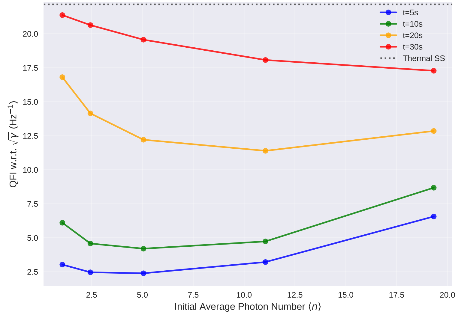
GKP QFI vs Initial Energy at Different Times
