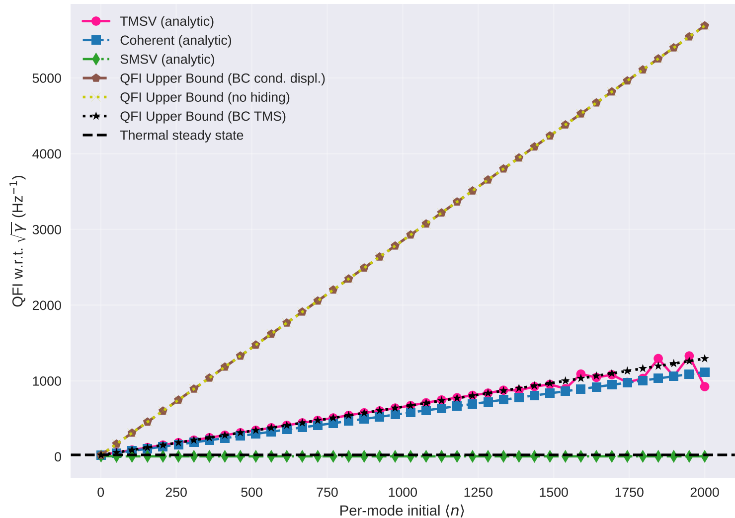
High-Energy QFI Comparison at t=10.0s
