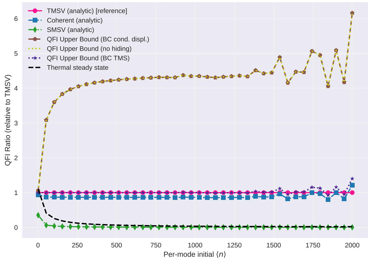
High-Energy QFI Comparison Normalized to TMSV at t=10.0s
