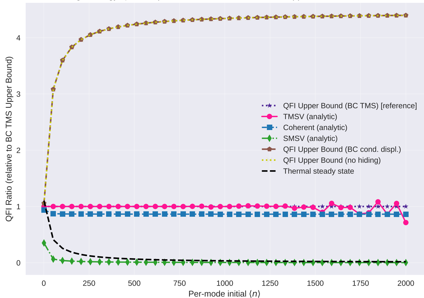
High-Energy QFI Comparison Normalized to BC TMS Upper Bound at t=10.0s
