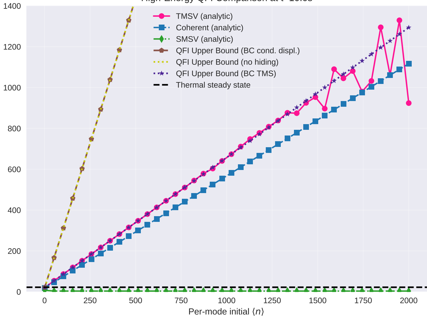
High-Energy QFI Comparison at t=10.0s
