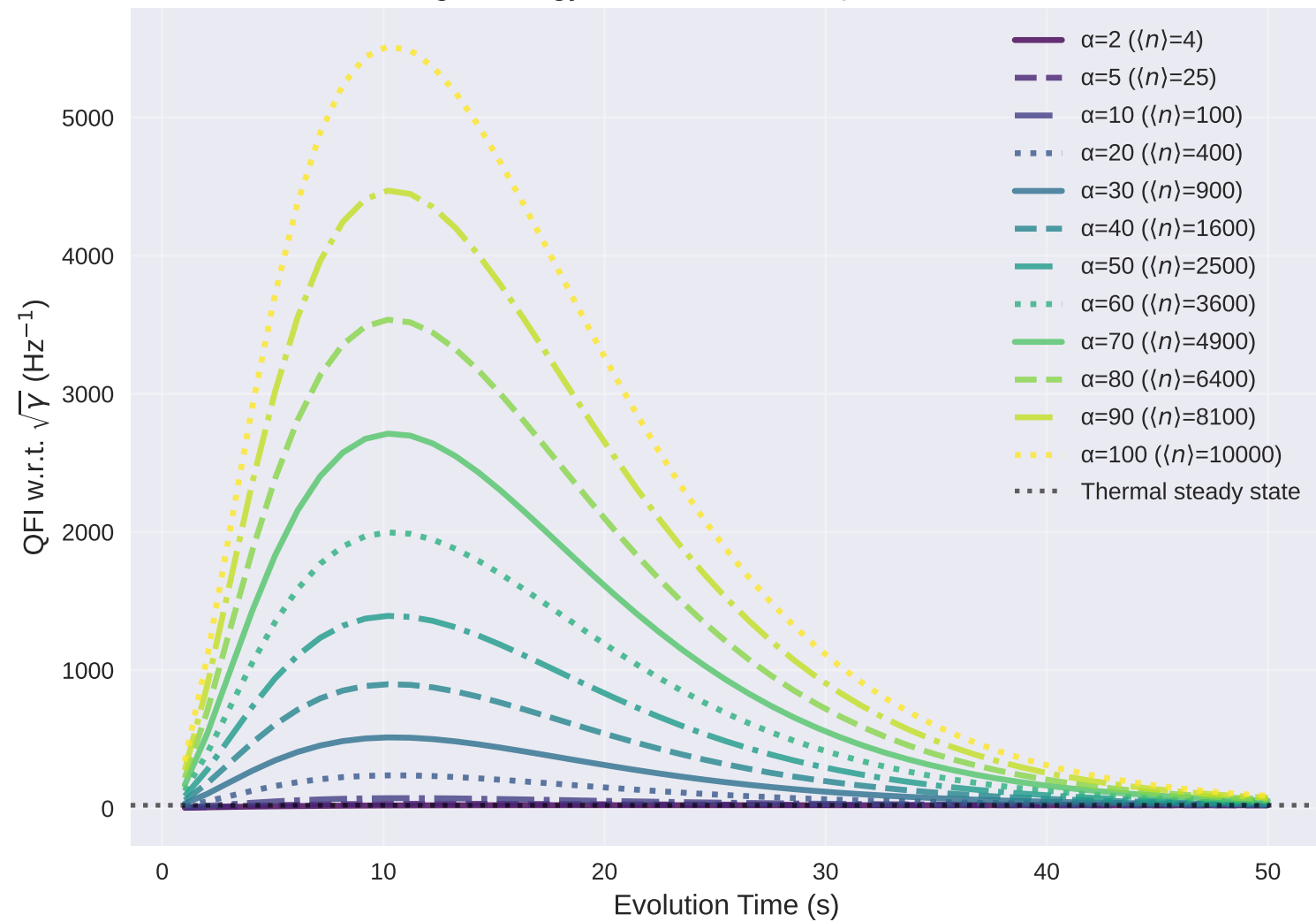
High-Energy Coherent State QFI: Different \alpha
