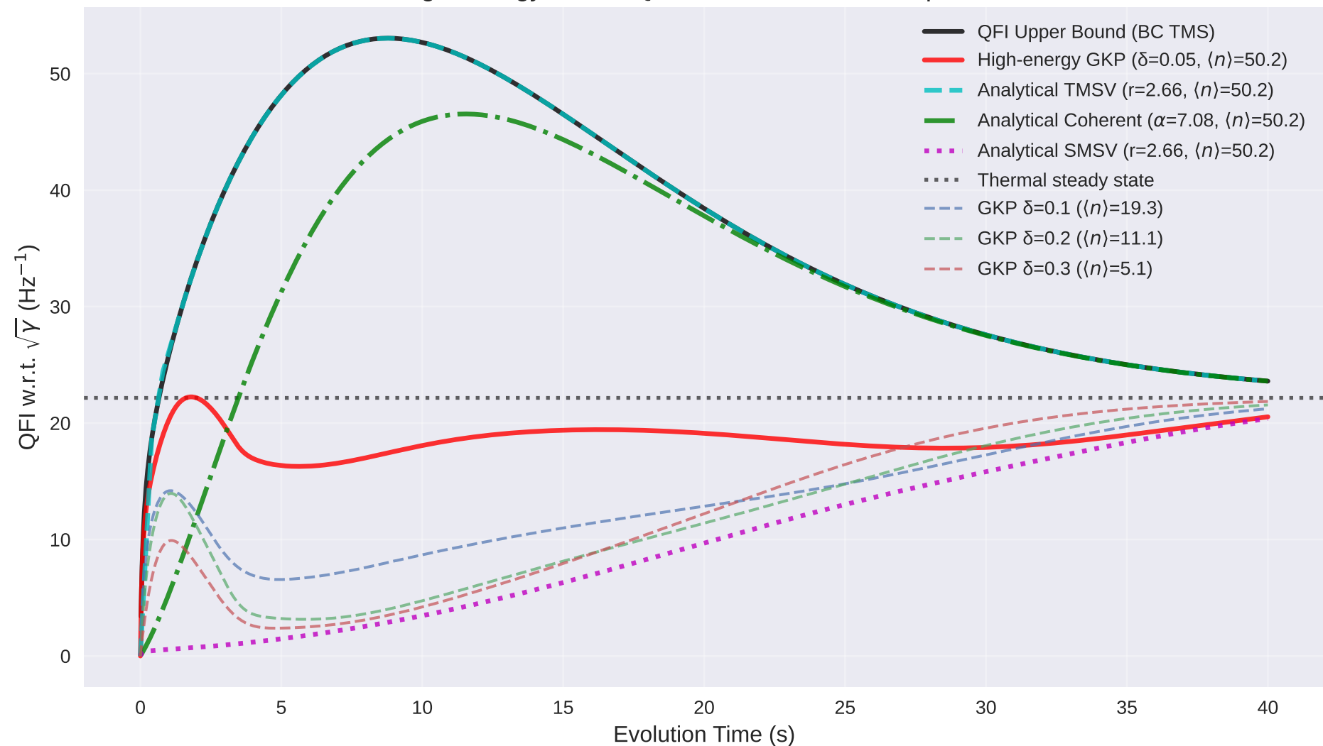
High-Energy States QFI: GKP vs TMSV Comparison
