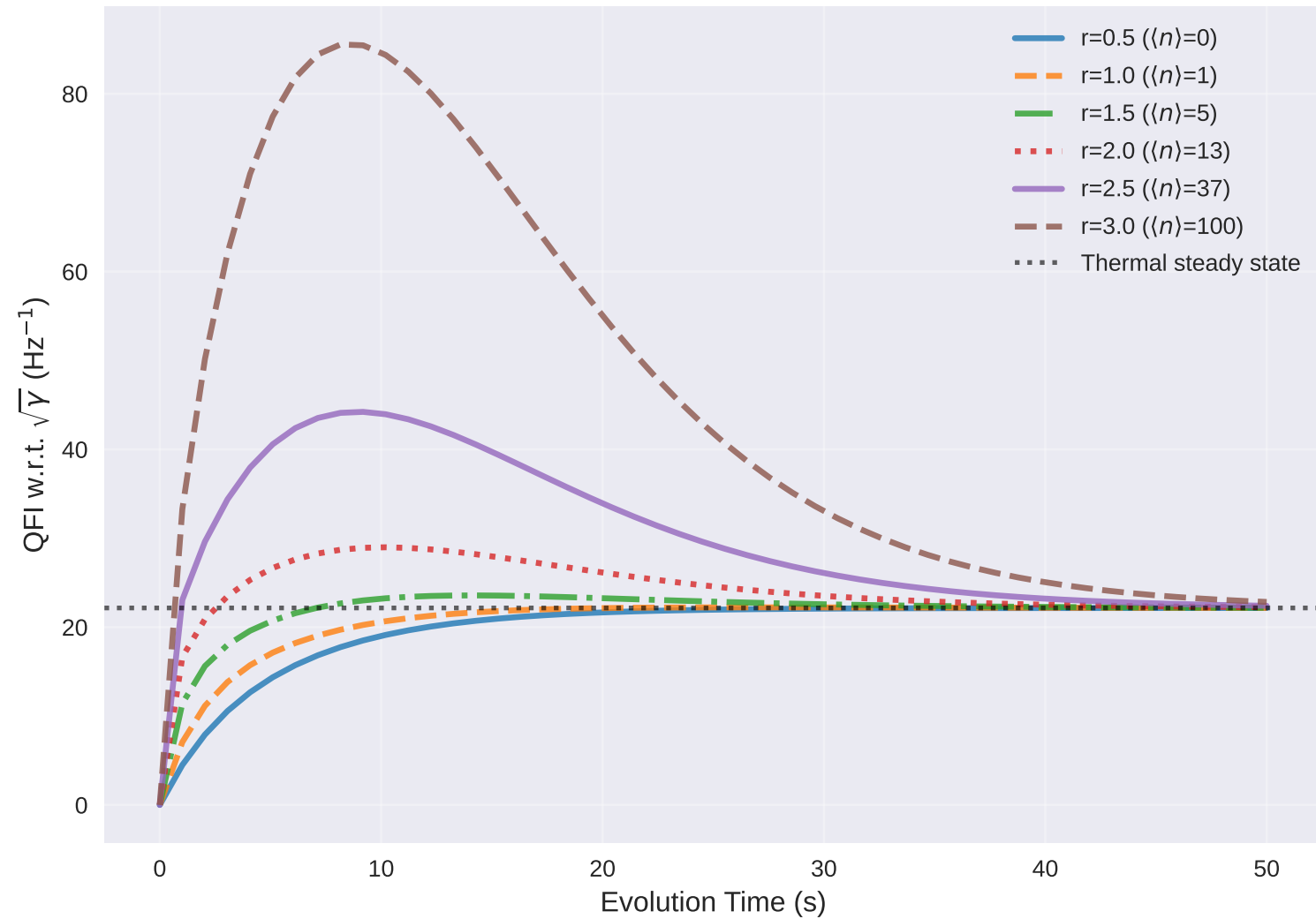
High-Energy TMSV QFI: Different Squeezing Parameters
