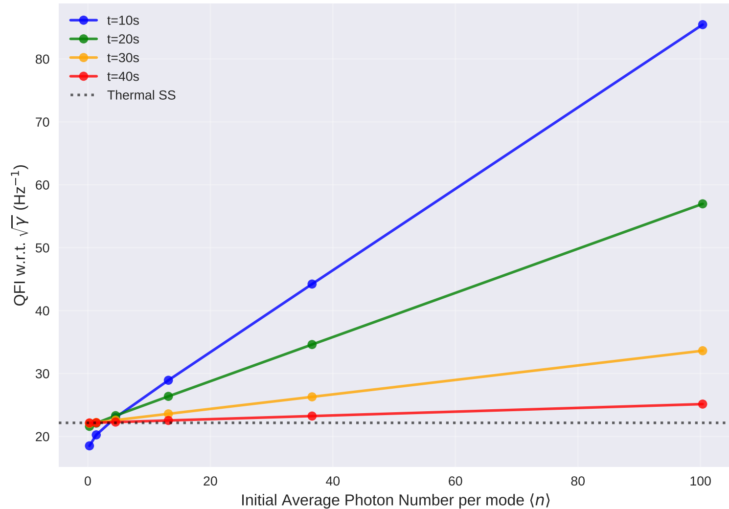
QFI vs Initial Energy at Different Times
