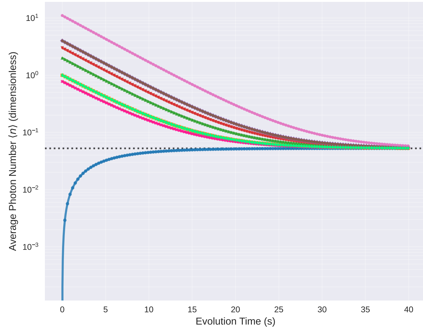
Average Photon Number vs Time (Log Scale)
