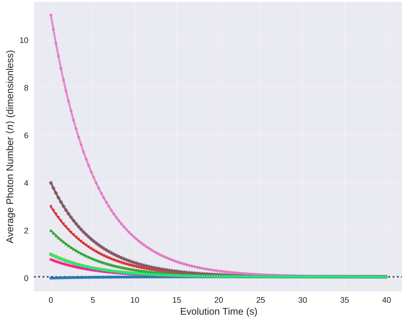
Average Photon Number vs Time
