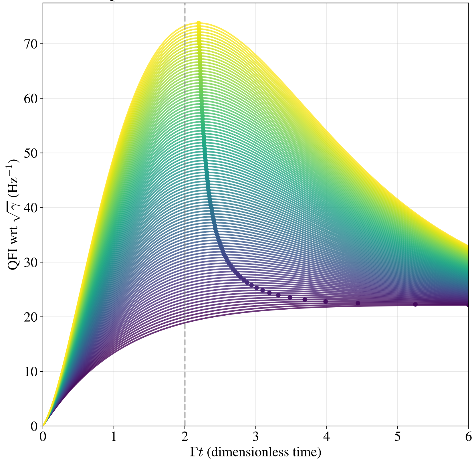
QFI of Coherent State vs Time for Different \bar{n}
