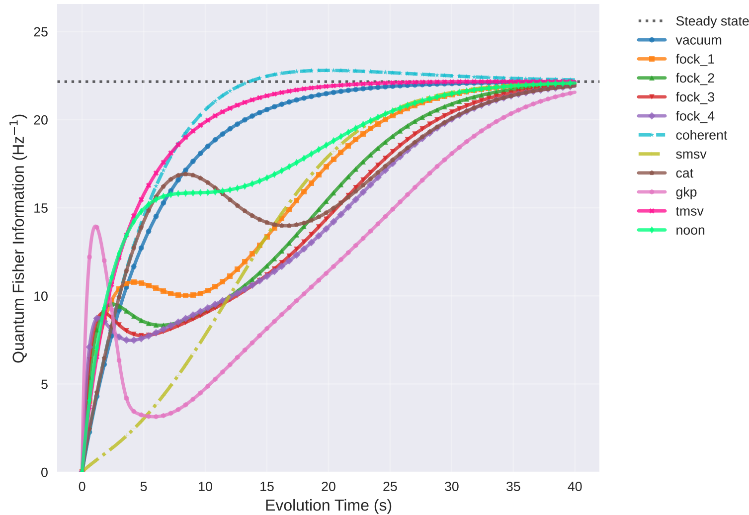
QFI w.r.t. \sqrt{\gamma} vs Time ( \gamma=0.01 Hz, \Gamma=0.2 Hz)
