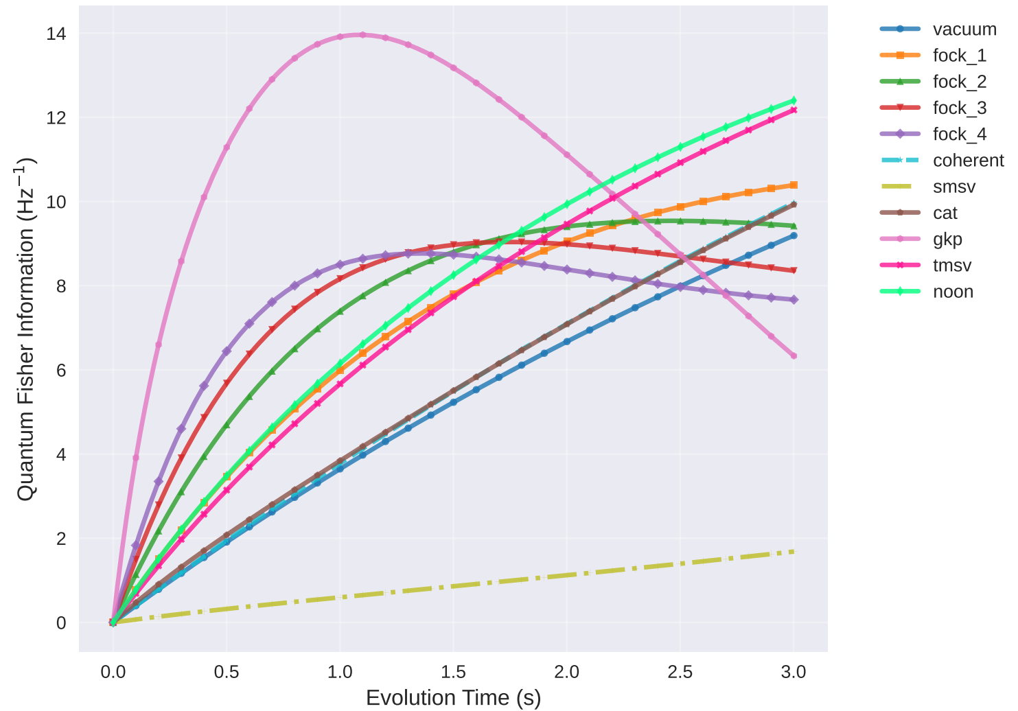
Early Time QFI Evolution
