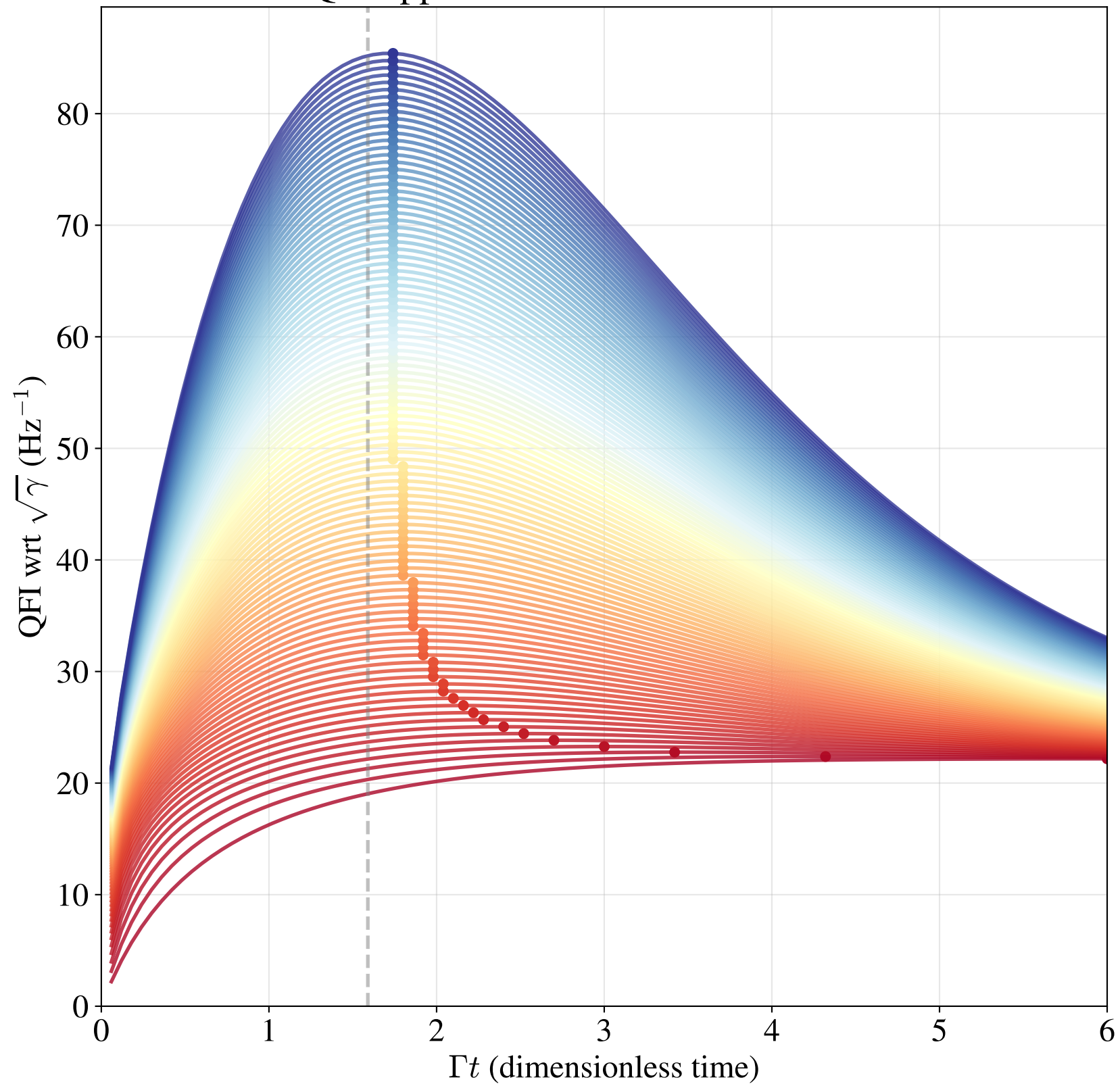
ECQFI upper bound vs Time for Different \bar{n}
