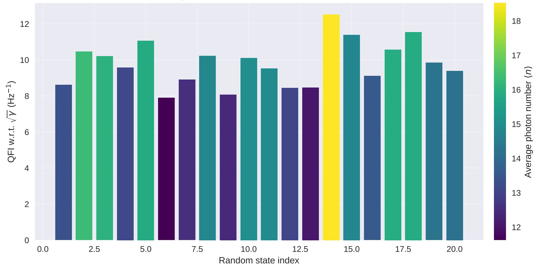
QFI of 20 Random States at t = 10.0s
