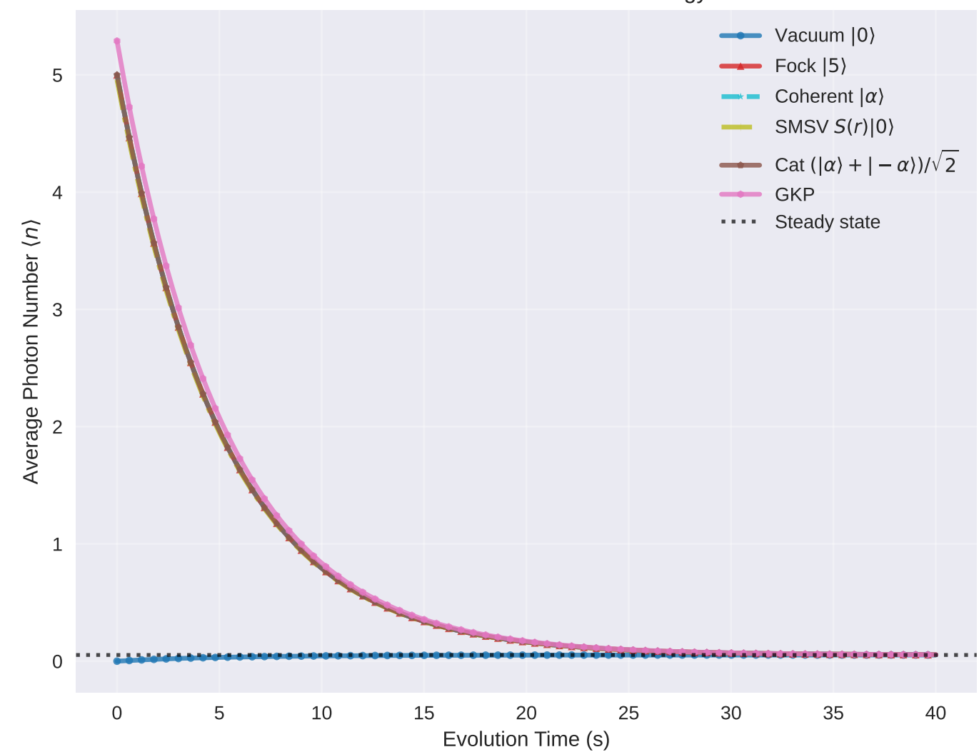
Photon Number Evolution: Same Initial Energy + Vacuum
