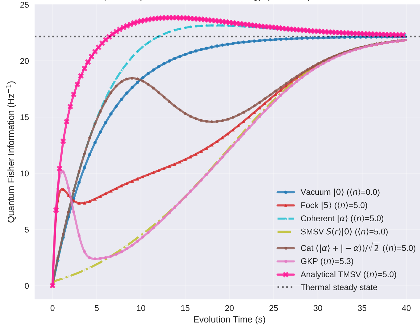
QFI Comparison: Same Initial Energy ( \langle n \rangle \approx 5.0 ) + Vacuum
