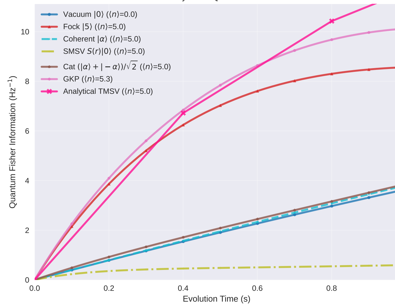
Early Time QFI Evolution
