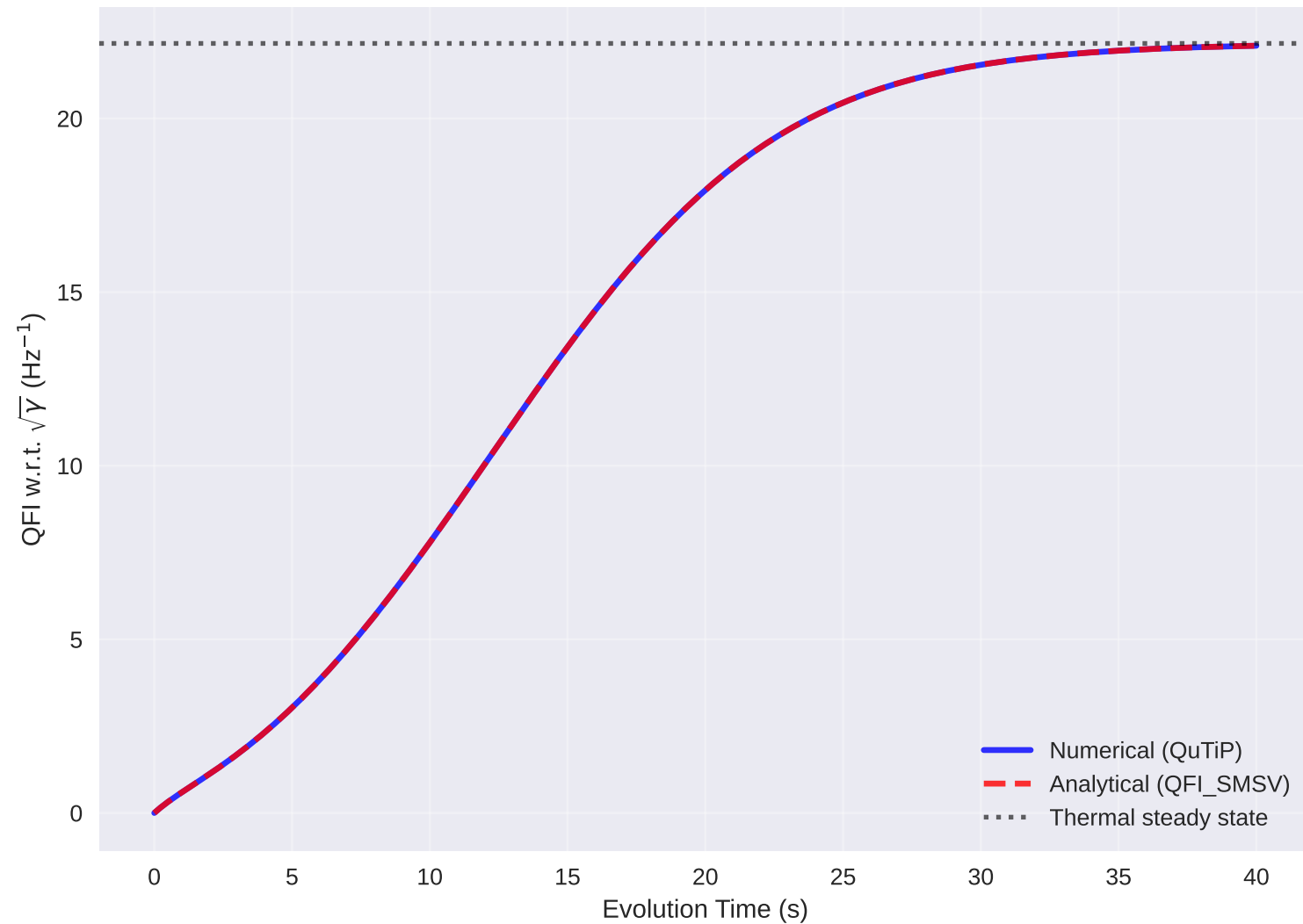
SMSV QFI: Numerical vs Analytical (r=0.8)
