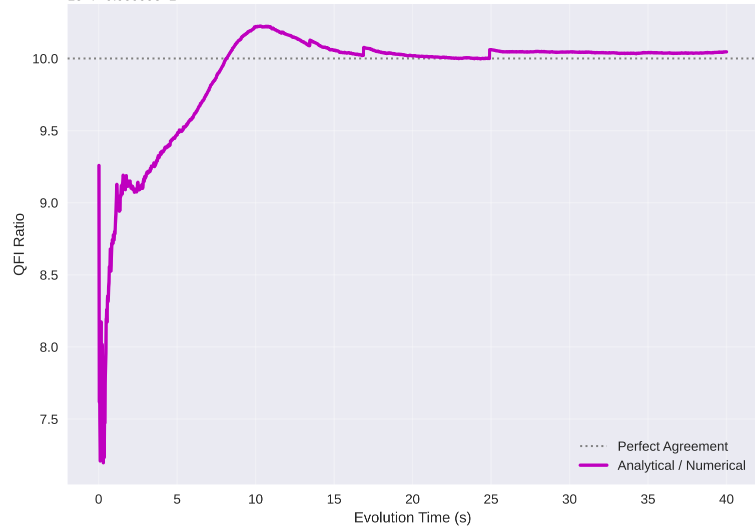
Ratio: Analytical / Numerical
