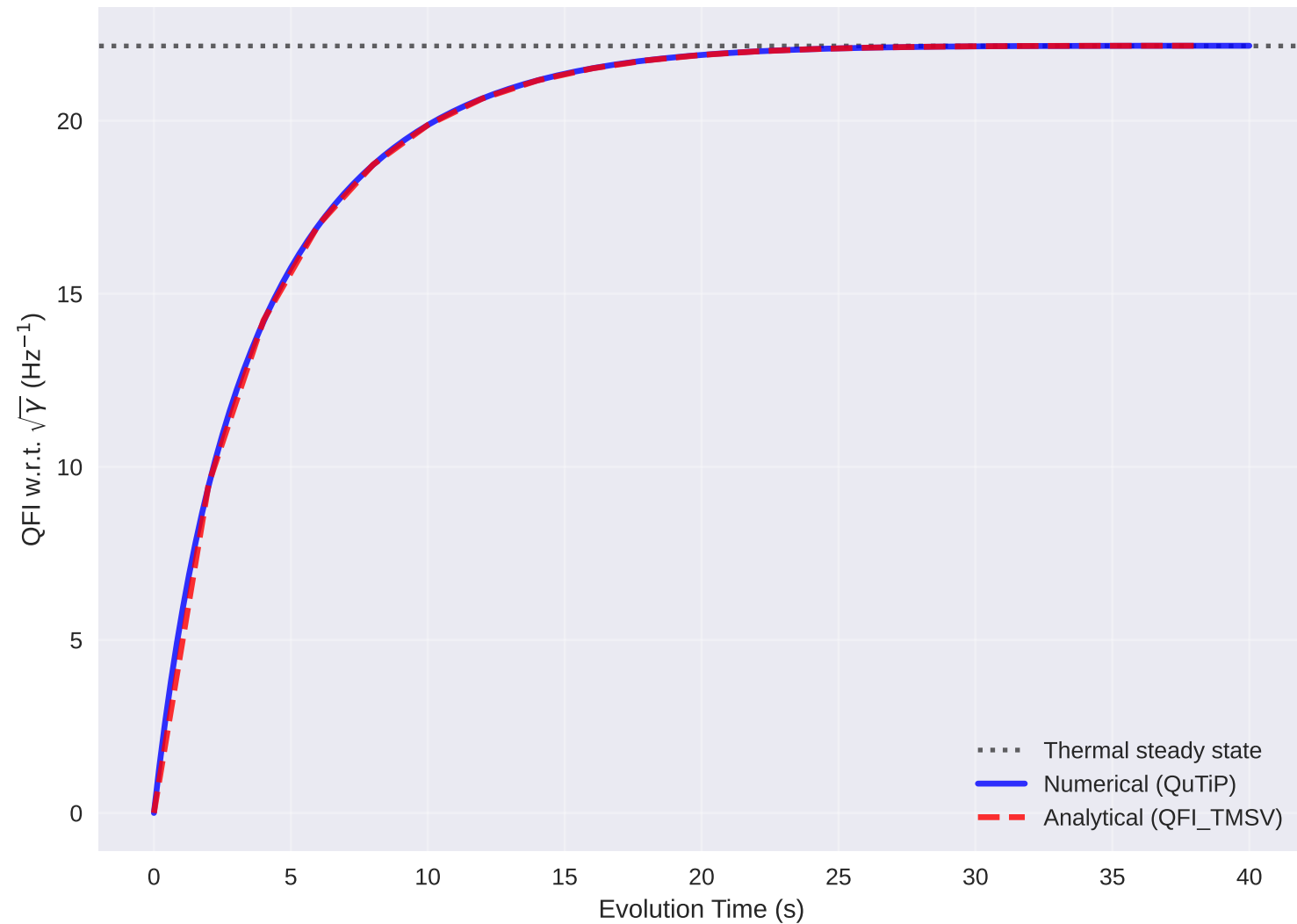
TMSV QFI: Numerical vs Analytical (r=0.8)
