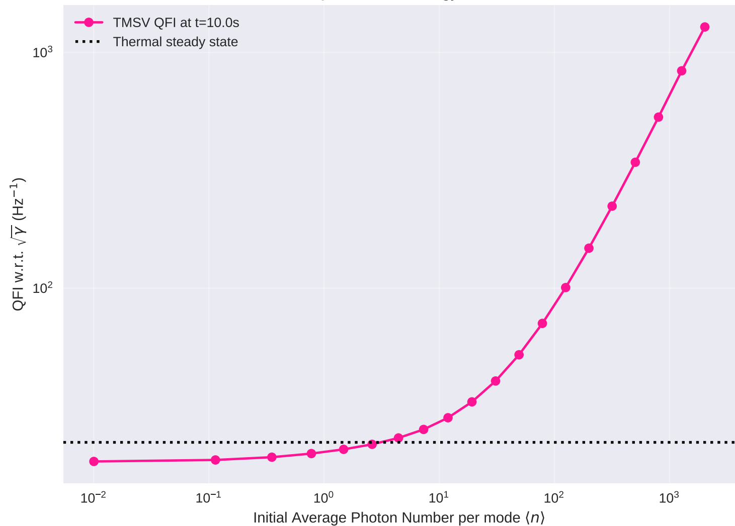
TMSV QFI vs Initial Energy at t=10.0s
