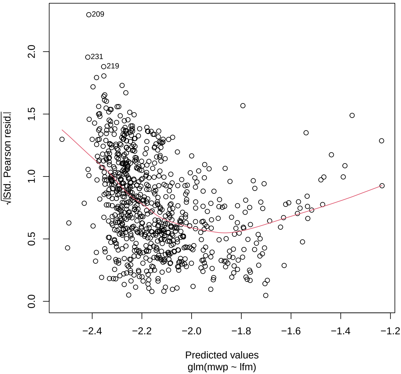
Scale-Location
