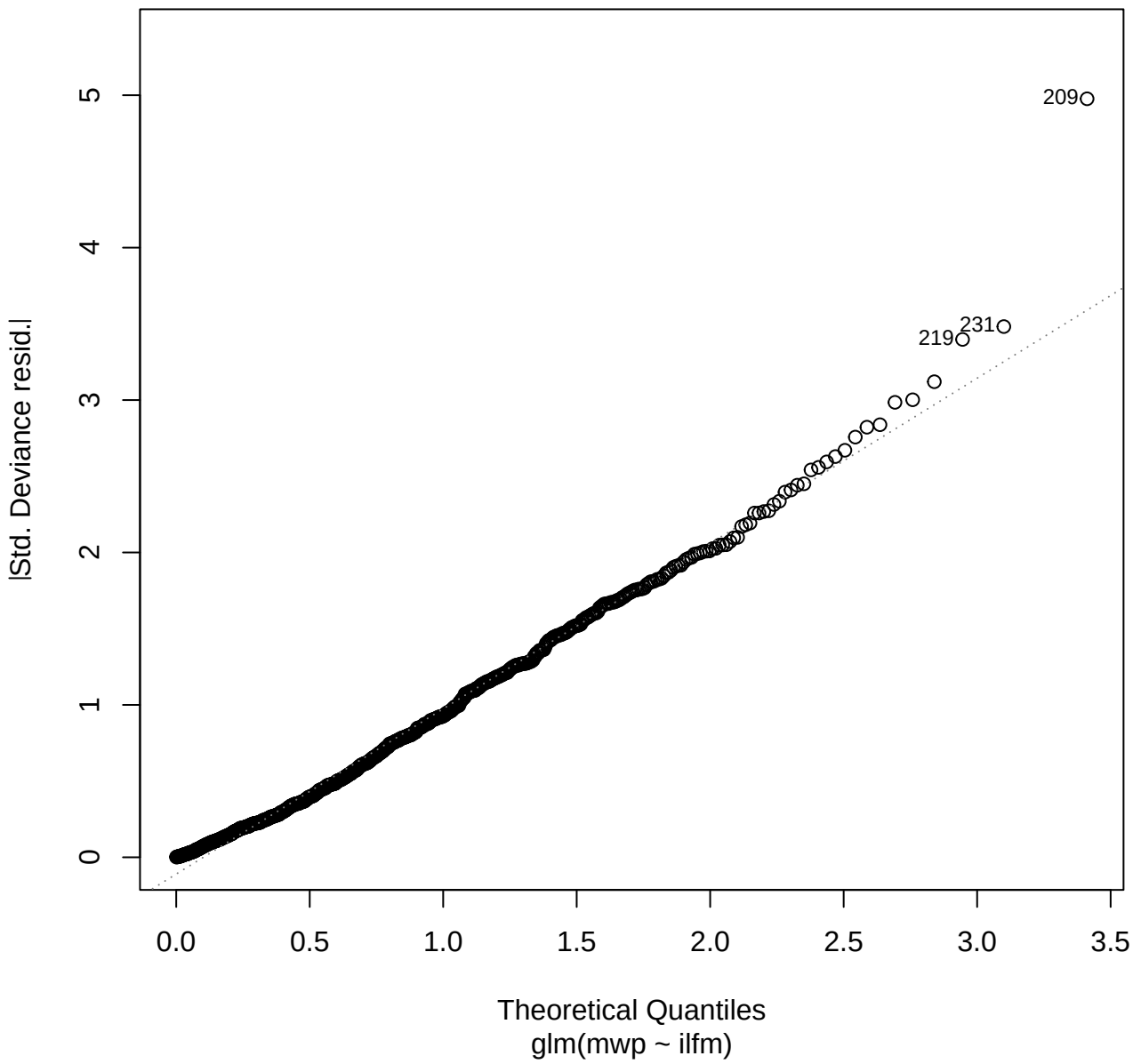
Q-Q Residuals
