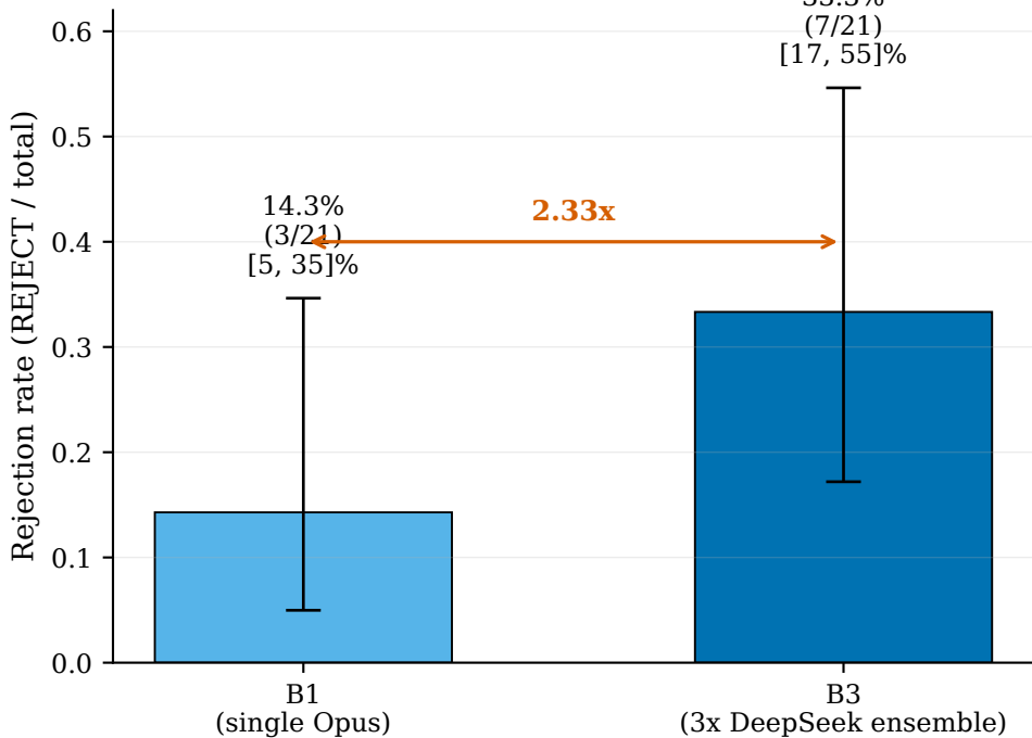
Figure 2. Critic-stage rejection rate on 21-class panel (Wilson 95% CI; B3 vs B1 ratio = 2.33x)
