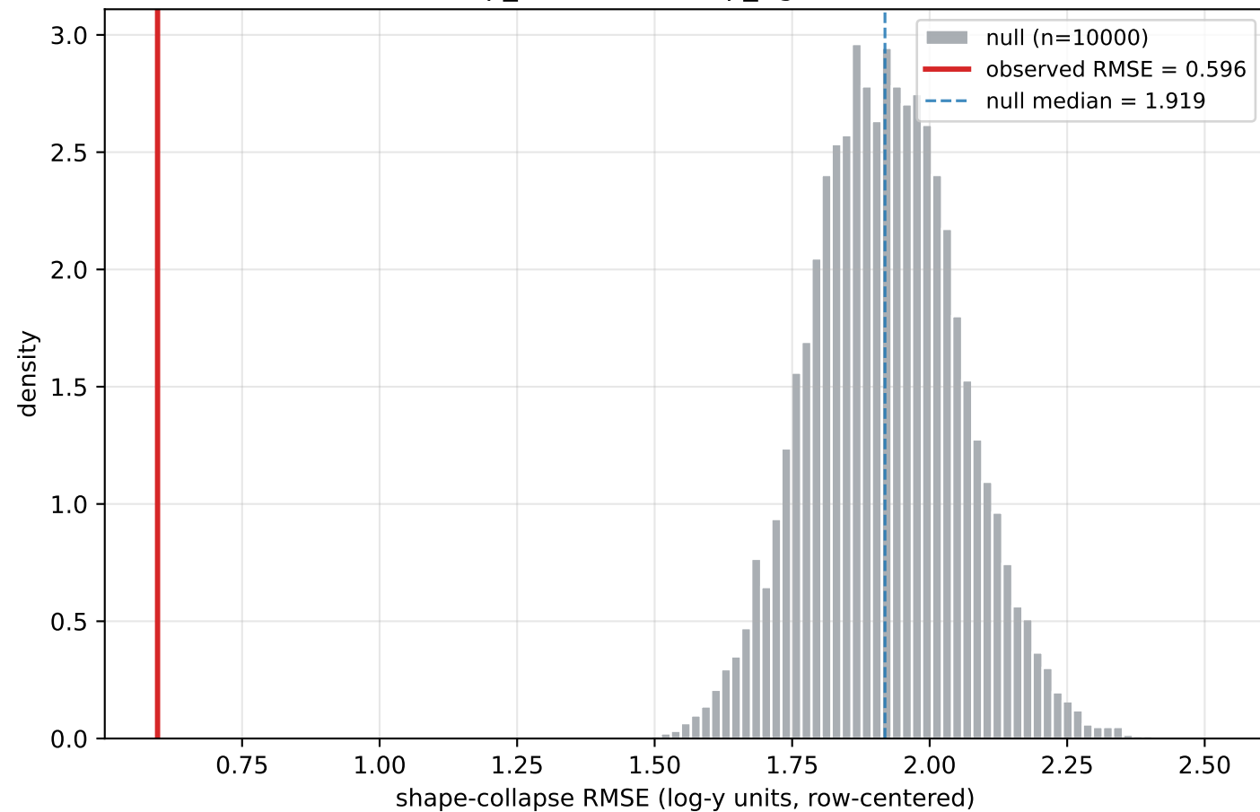
(a) Shape-collapse RMSE vs Gaussian-surrogate null
