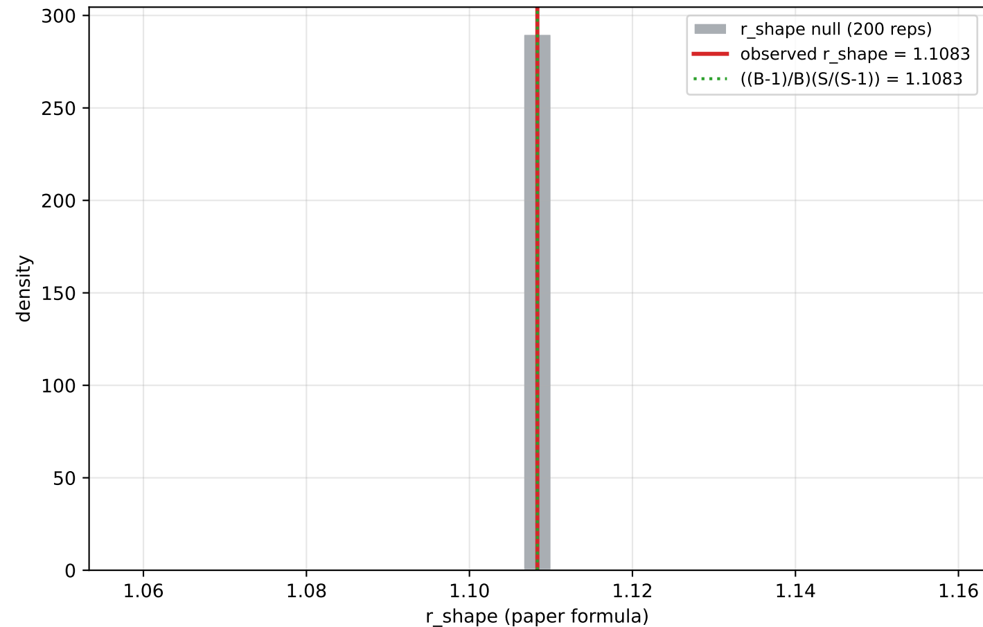
(b) Paper's r_shape statistic is a combinatorial artifact
