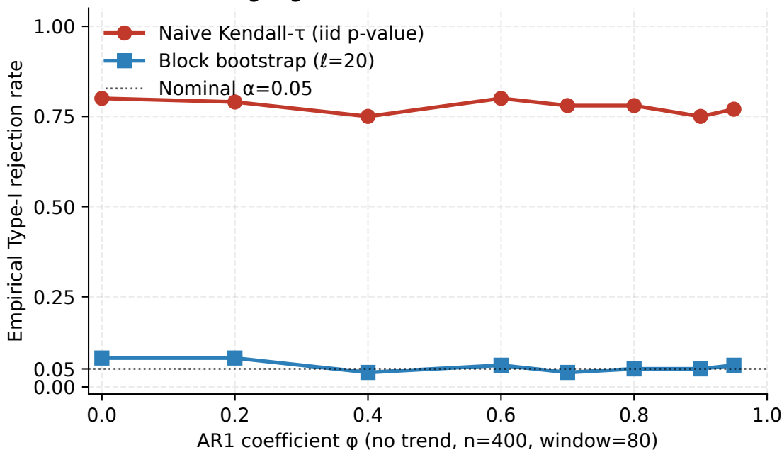
Type-I inflation of naive Kendall- \tau vs block-bootstrap on rolling lag-1 autocorrelation under AR1 noise
