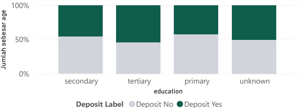
Eductions Impact
