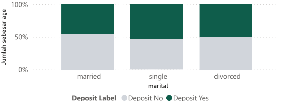
Marital Impact
