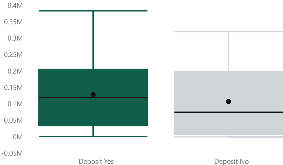
Balance Impact
