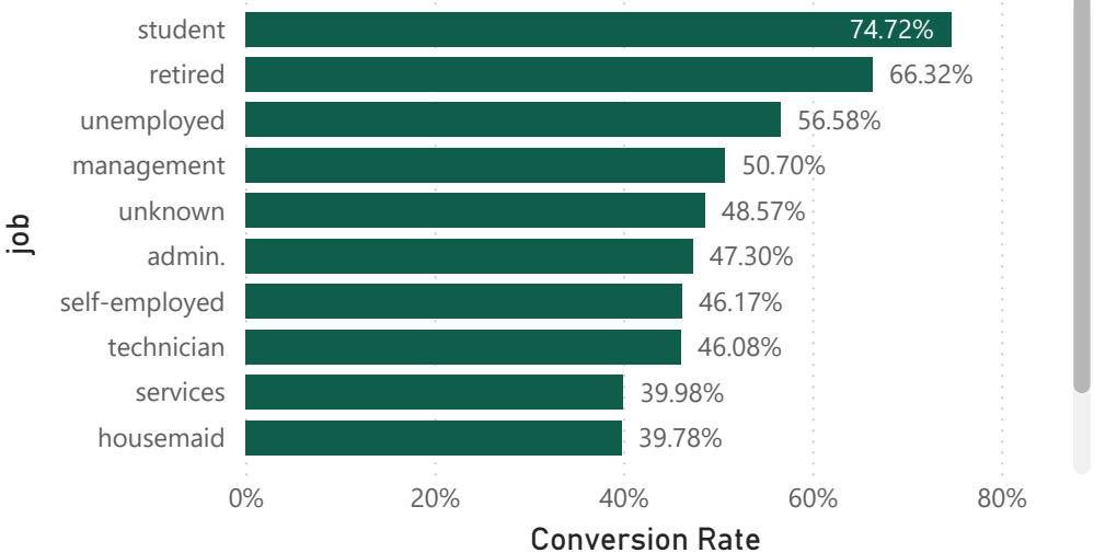
Job Impact
