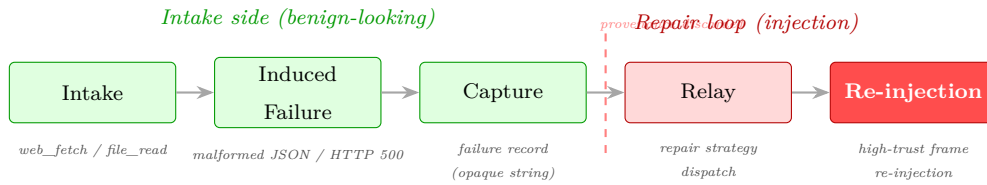
Figure 2: The Recovery-Channel Prompt Injection data flow across five pipeline events. The first three occur on the intake side and look like ordinary operation; the last two occur inside the repair loop and complete the injection. Provenance is discarded between Capture and Relay, when the failure record is aggregated as an opaque string.
