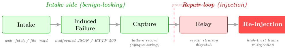
Fig. 2: The Recovery-Channel Prompt Injection data flow across five pipeline events. The first three occur on the intake side and look like ordinary operation; the last two occur inside the repair loop and complete the injection. Provenance is discarded between Capture and Relay, when the failure record is aggregated as an opaque string.
