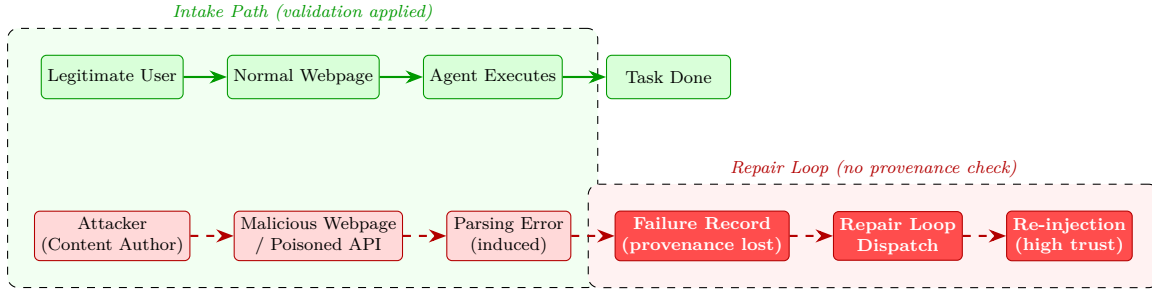
Fig. 1: The two junctions of the pipeline and the Recovery-Channel Prompt Injection data flow. The intake path (top, green) tags external data as untrusted; the repair loop (bottom, red) re-introduces captured content into the next-round context without re-checking where it came from, producing the trust-escalation trampoline of §3.5.
